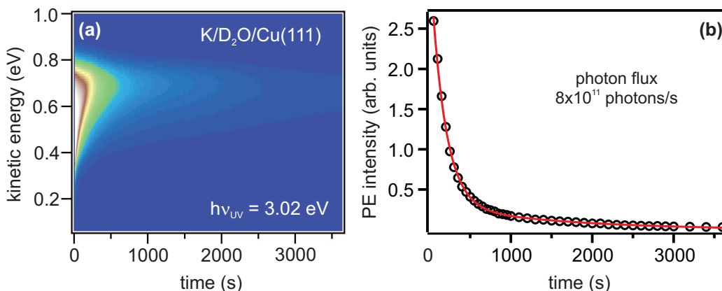
Figure 4.18: Depopulation of the K 4s state. (a): False-color plot of the PE intensity as a function of illumination time. The sample is irradiated with a fluence of 8 \cdot 10^{-5} J/cm^2 by UV photons with a photon energy of h\nu = 3.02 eV. (b): Peak intensity of the direct PE peak as a function of illumination time. The data is fitted by a bi-exponential decay (solid red line). The initial decay rate is 5.7(2) \times 10^{-3} s^{-1} followed by a significantly slower decay with a rate of 6.4(2) \times 10^{-4} s^{-1} . The photon flux is 8 \cdot 10^{11} \frac{\text{photons}}{s} .
