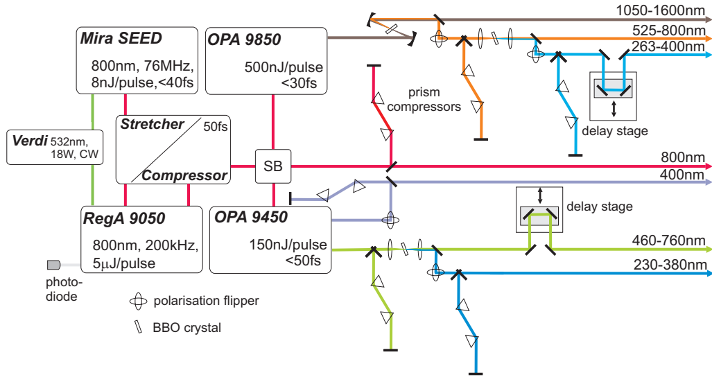
Figure 3.7: Laser System
