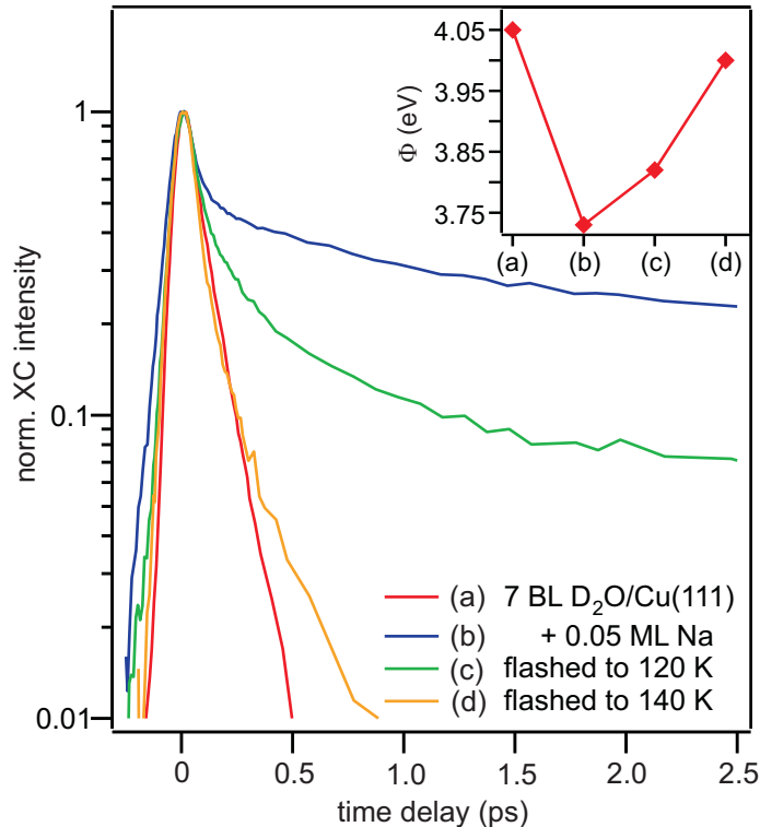
Figure 4.16: Incorporation of Na ions in amorphous D 2 O ice. (Main panel): XC traces for amorphous 7 BL D 2 O ice ((a), red line) and for 0.05 ML Na coadsorbed on top of the amorphous ice film ((b), blue line). Temperature flashes to 120 and 140 K and subsequent cooling of the sample to T≈60 K, ((c), green line) and ((d), yellow line), respectively, lead to an increase of the population dynamics. (Inset): Work function \Phi of the sample for the indicated steps (a)-(d) of the experiment. See text for details.
