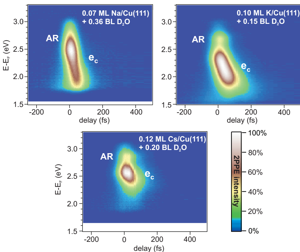
Figure 5.11: Time-resolved 2PPE data of different alkali/water clusters on Cu(111). 2PPE intensity in false color representation as a function of intermediate state energy (left axis) and pump-probe delay (bottom axis). The spectra for Na, K, and Cs exhibit a short-lived state attributed to the alkali resonance and a broader feature shifting to lower energies with increasing time delay, which is associated with excess electrons at the alkali/water cluster.
