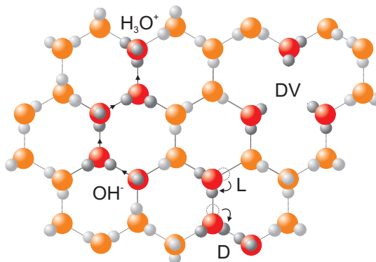
Figure 2.17: Schematic presentation of protonic point defects in ice I_{ce_h} . Ionic defects form when the first ice rule is broken, Bjerrum defects occur when the second ice rule is violated. If a water molecule is missing in the lattice a dressed vacancy is present. (from left to right)
