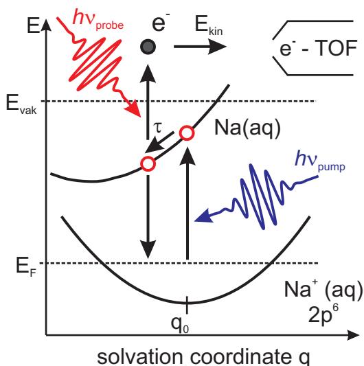
Figure 4.1: Scheme of the 2PPE experiment for solvation in Na/D_2O/Cu(111) . The excitation of an electron by absorption of a photon with h\nu_{pump} leads to (i) an attachment of the electron to the Na 3s state resulting in the neutralization of the alkali or (ii) the formation of a Na^+(D_2O)_n^- complex. The transient electron population is then probed by absorption of a second photon with h\nu_{probe} .
