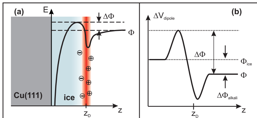
Figure 4.19: Influence of the surface dipole layer on the systems work function. (a): Side view of the layer structure of K/D 2 O/Cu(111). At the ice/vacuum interface a distance z_D to the surface plane a dipole layer is formed by the positively charged alkali ions and the surrounding water molecules that screen the ions. The image potential is modified such that potential minima occur at the interface. (b): Dipole potential \Delta V_{dipole} as a function of the distance to the surface z . The dipole layer at the surface leads to a repulsive and an attractive part of the potential for electrons that propagate through the dipole layer. The minimum energy for an electron, that passes through this layer, needed to overcome the systems work function \Phi is increased by \Delta\Phi . See text for details.
