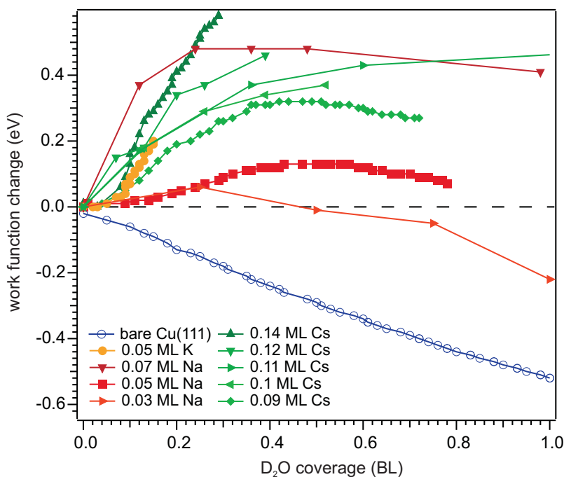
Figure 5.3: Relative work function change versus D 2 O coverage for various pre-coverages of Na, K, and Cs. The water was dosed at 35 K. The blue circles represent data obtained by deposition of D 2 O on clean Cu(111).
