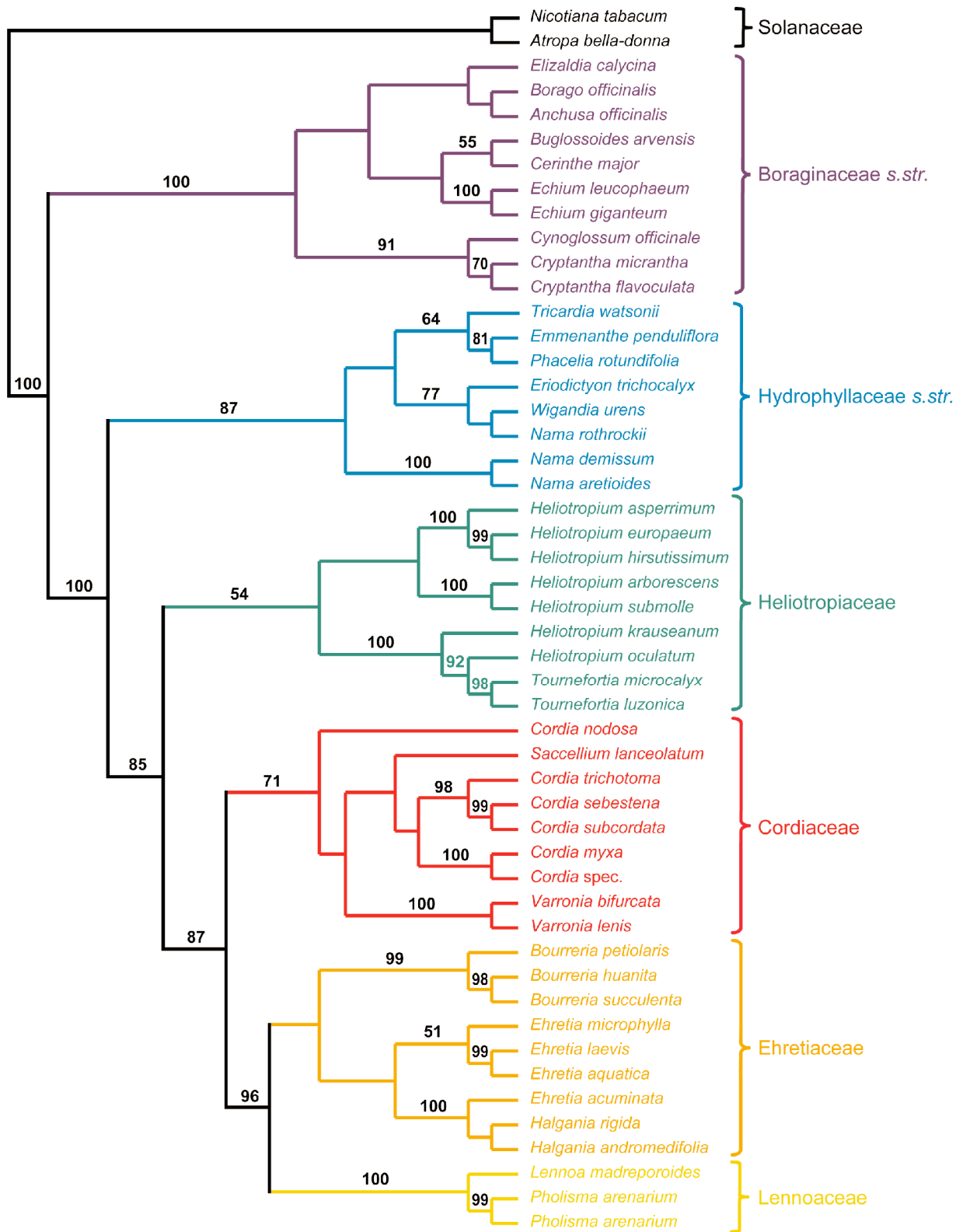
Figure 3-10: One of five most parsimonious trees of Boraginales (L = 383, CI = 0.50, RI = 0.65). Important taxa are indicated. The numbers above branches are bootstrap support values to the clusters to the right of them (percentages under 50% not shown).
