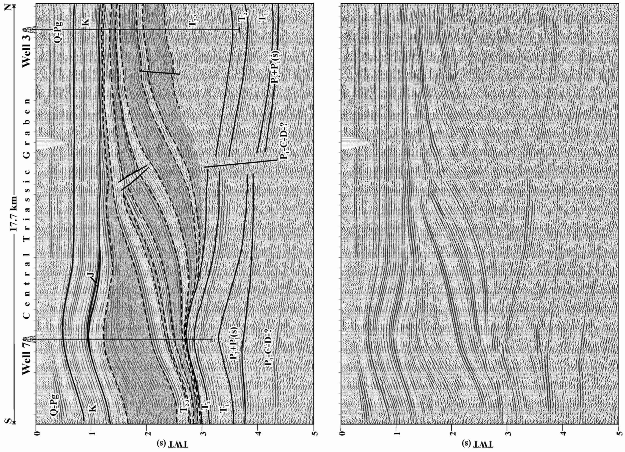
Seismic line 12
