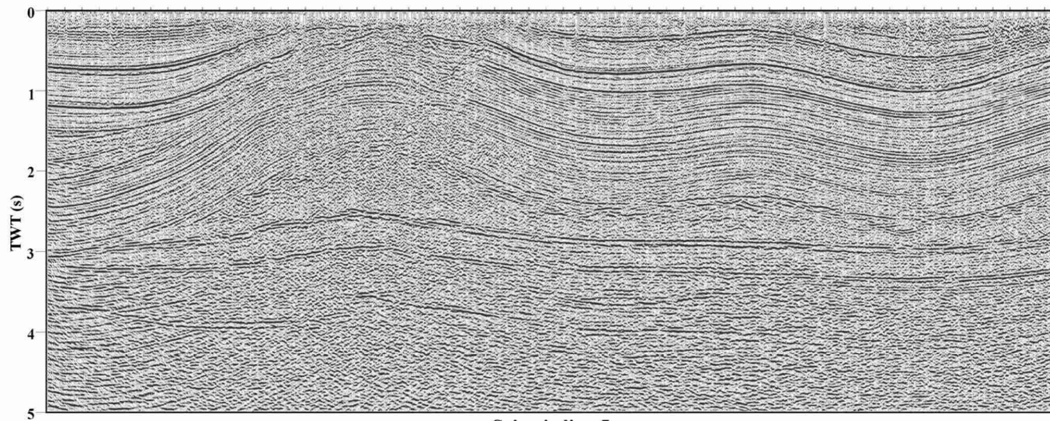
Seismic line 5
