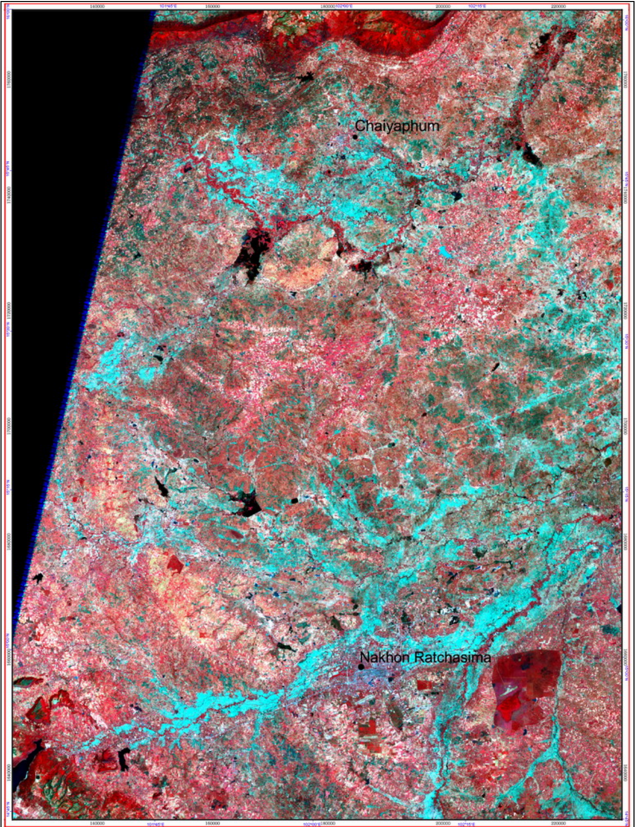
False Color Composite Image Landsat 7 ETM+ (27.12.1999) Western Khorat Plateau, NE Thailand Bands 4, 3, 2 as red, green, blue
