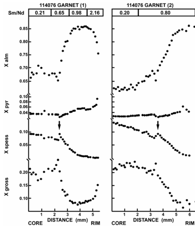
Fig. 6.12: Compositional profiles across two garnet megacrysts from Stuckless Cove (Newfoundland) (Vance and O’Nions, 1990). Garnet 1 shows a marked compositional break between core and rim, which is not visible in garnet 2. Both profiles show an increase in Ca and Mn which coincides with the compositional break in garnet 1 (arrows). See text for discussion.
