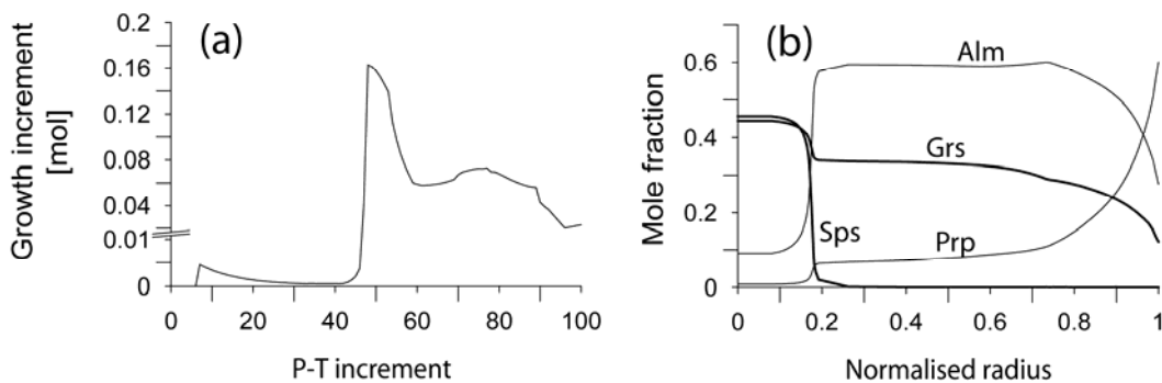
Fig. 6.6: Garnet growth increment (a) and calculated zonation pattern (b) for growth along the P-T segment assuming decreasing manganese availability for the garnet surface. Note the decreasing growth increment between initial garnet formation and the peak near point 50. The calculated zonation pattern shows steep compositional gradients caused by limited garnet growth due to disequilibrium element incorporation.
