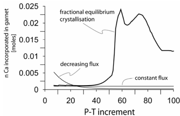
Fig. 6.2: Amount of calcium incorporated in the garnet edge at every calculated step. The bold curve shows the incorporated Ca-amount calculated for fractional equilibrium crystallisation, the two other curves display the limited amount available for the garnet edge for the two different disequilibrium crystallisation scenarios (see text).
