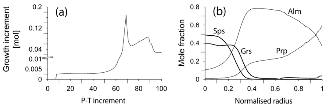
Fig. 6.7: Garnet growth increment (a) and calculated zonation pattern (b) for growth along the P-T segment assuming constant calcium availability for the garnet surface. Disequilibrium incorporation of calcium enlarges the stability field of chlorite (shifted peak in (a)) and causes a characteristic intervening increase in grossular content in the calculated zonation pattern (b).
