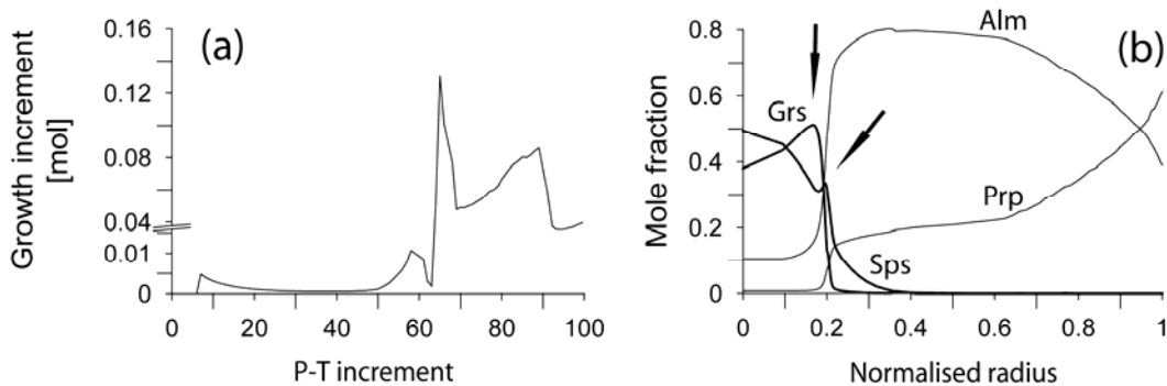
Fig. 6.8: Garnet growth increment (a) and calculated zonation pattern (b) for growth along the P-T segment assuming decreasing calcium availability for the garnet surface. Limited calcium supply leads to repeated decrease in growth increment (arrow in a) and a characteristic rise in grossular accompanied by an intermediate rise in spessartine components (arrows in b).
