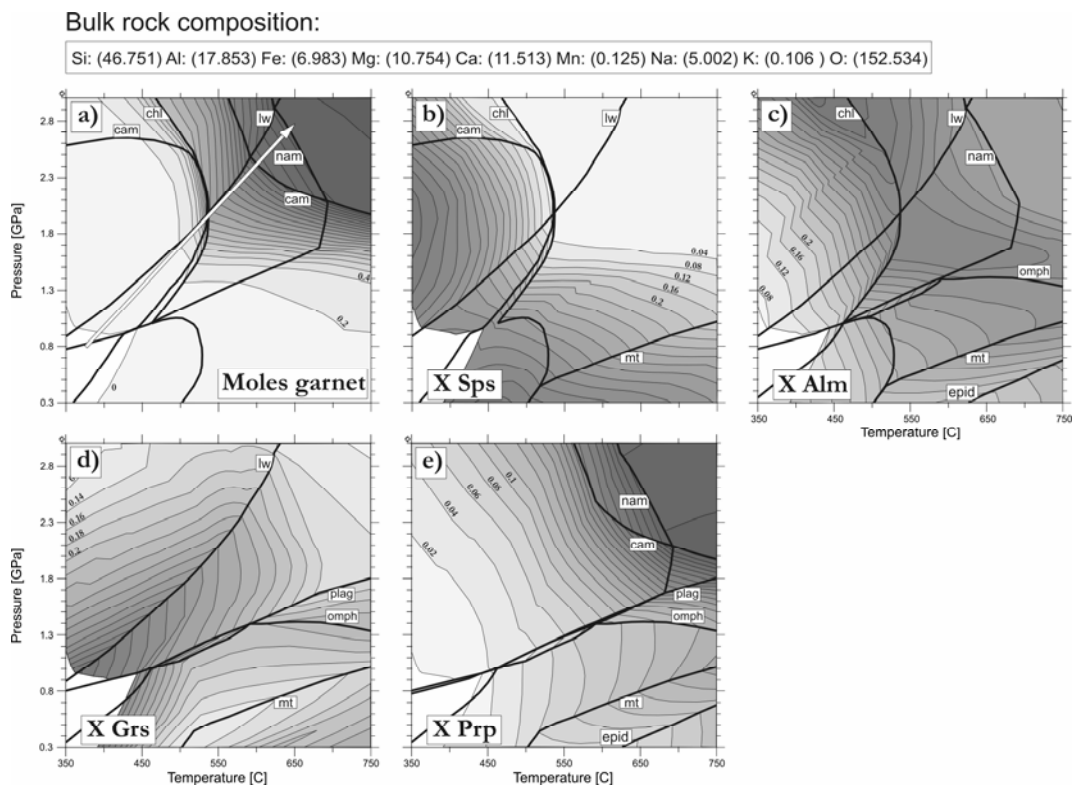
Fig. 6.3: Garnet mode (a), composition (b-e) and mineral isograds most influencing garnet composition for an average basaltic rock in the water saturated NCKFMASHMn system. Darker colours display higher mole fractions. The arrow marks the P-T segment along which garnet evolution is modelled.
