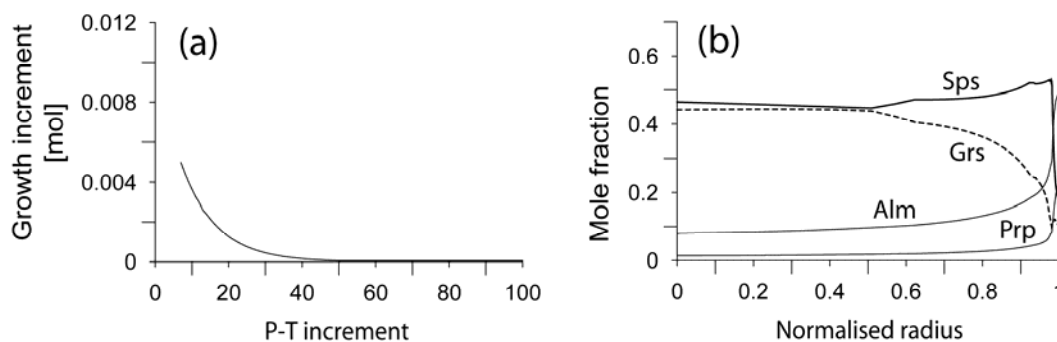
Fig. 6.10: Garnet growth increment (a) and calculated zonation pattern (b) for growth along the P-T segment assuming decreasing aluminium availability. Due to the rapidly decreasing growth increment, the compositional break occurs only at the outermost rim (b).
