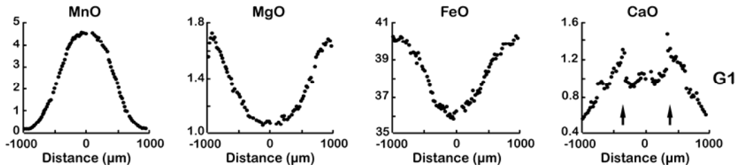
Fig. 6.13: Compositional profile across a garnet crystal from Pecuris Range, New Mexico, USA (redrawn after Chernoff and Carlson, 1997). Note the sudden rise of CaO due to disequilibrium incorporation of calcium (arrows).
