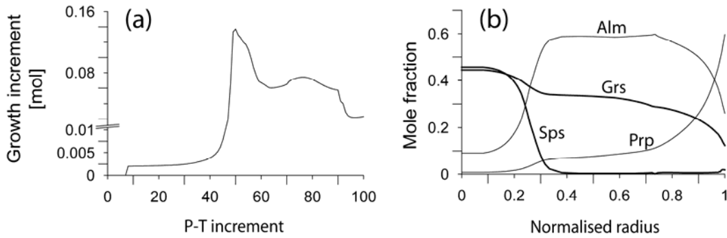
Fig. 6.5: Garnet growth increment (a) and calculated zonation pattern (b) for growth along the P-T segment assuming constant manganese availability for the garnet surface. The peak in (a) resulting from chlorite consumption is shifted, compared to calculations assuming equilibrium crystallisation, indicating the influence of disequilibrium garnet growth on the mineral assemblage.
