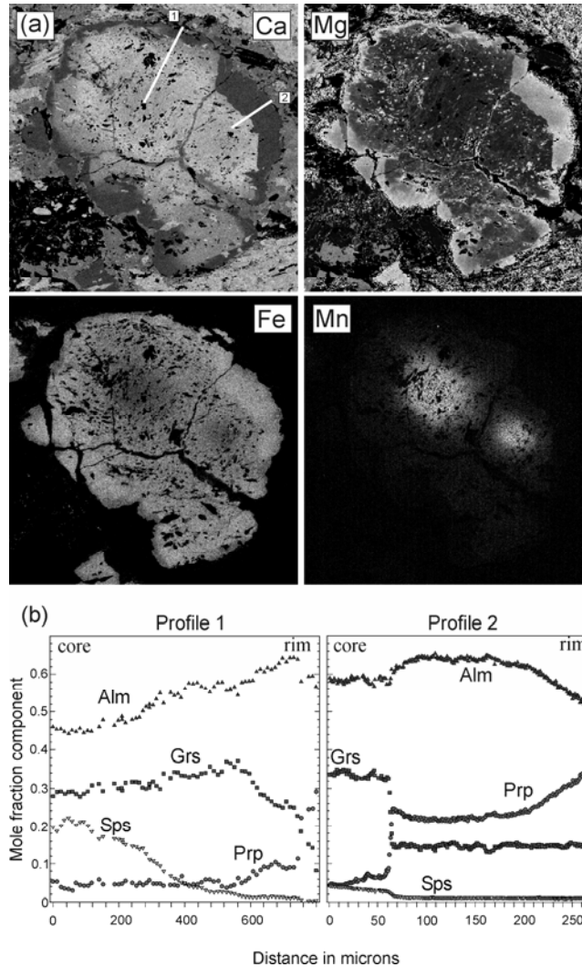
Fig. 6.11: Compositional mapping (a) and compositional profiles (b) of a garnet aggregate from the Tso Morari area (Western Himalaya). (a) The Fe- and Mn- maps show that the garnet is a composite of two amalgamated grains. The lines mark the position of the profiles (1 and 2) in Fig. 6.7b. Profile 1 shows a continuous compositional gradient, whereas profile 2 shows a discrete compositional change at the interface of the core and rim (see text).
