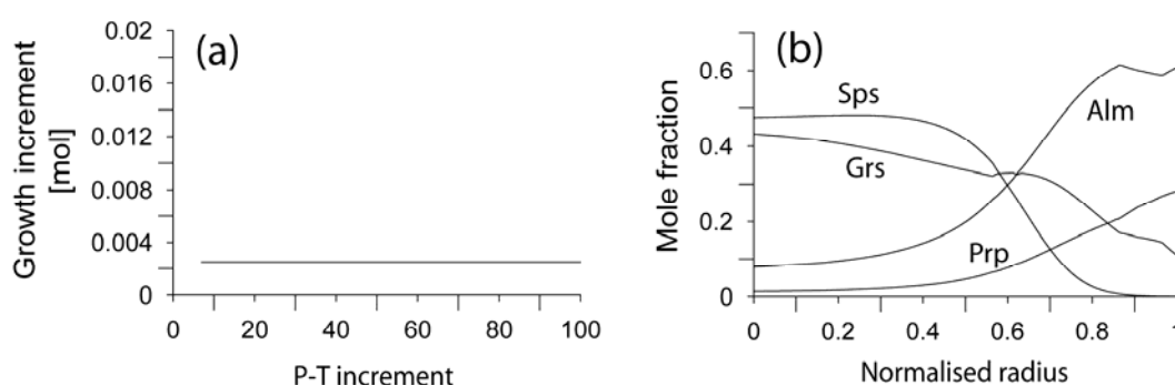
Fig. 6.9: Garnet growth increment (a) and calculated zonation pattern (b) for growth along the P-T segment assuming constant aluminium availability. In this case garnet growth is directly related to the amount of Al available for the garnet surface. The resulting zonation pattern (b) does not show the strong increase in pyrope content accompanied by a decrease in the almandine component at high pressures.
