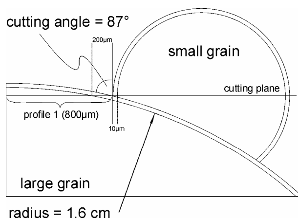
Fig. 6.14: Schematic illustration of a textural relation between the two garnets in Fig. 6.11, that might possibly lead to a misinterpretation of the observed compositional profiles (see text for discussion).
