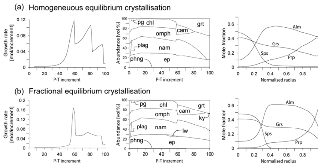
Fig. 6.4: Garnet growth increments, mineral abundances and modelled garnet zonation patterns for (a) homogeneous and (b) fractional equilibrium crystallisation along the P-T segment shown in Fig. 6.2a. The step-like garnet growth in (a) is caused by progressive consumption of chlorite, calcic and sodic amphibole.
