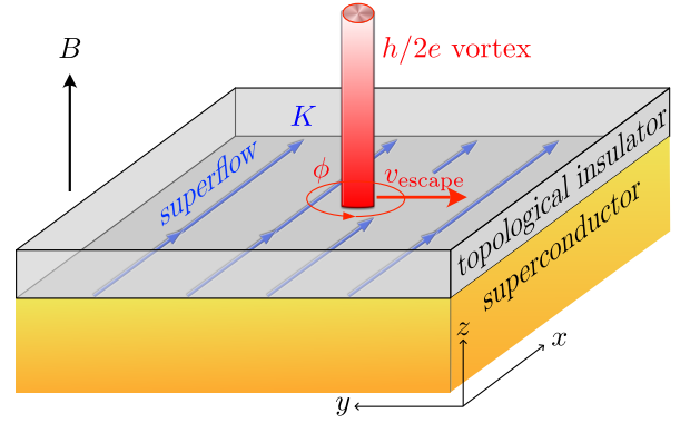
FIG. 1. Schematic of a topological insulator with induced superconductivity (gap \Delta_0 ) in a perpendicular magnetic field B . A vortex (red, with a 2\pi winding of the superconducting phase \phi ) binds a Majorana zero-mode. An in-plane supercurrent (blue arrows, Cooper pair momentum K ) can deconfine the zero-mode, producing a Majorana fermion wave packet that escapes with velocity v_{\text{escape}} in a direction perpendicular to the superflow.
