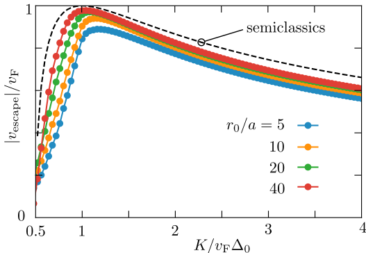
FIG. 5. Escape velocity of a zero-mode wave packet from the vortex core, as a function of the superflow momentum K . The data points follow from the computer simulation, for different core sizes r_0 (at fixed \Delta_0 = 0.2 v_F/a ). The black dashed curve is the semiclassical result (4.9).
