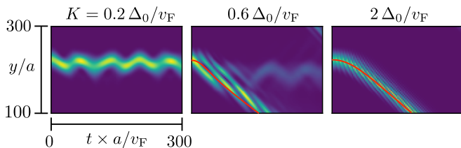
FIG. 4. Propagation of the zero-mode along the y -axis after the superflow momentum quench at t = 0 . The color scale shows the density profile \int |\Psi(x, y, t)|^2 dx following from the computer simulation ( \Delta_0 = 0.2 v_F/a , r_0 = 40 a , B = (h/e)(302 a)^{-2} ). The red curve results from integration of the semiclassical equation of motion (4.10), for the same \Delta(r) = \Delta_0 \tanh(r/r_0) gap profile as in the numerics [24].
