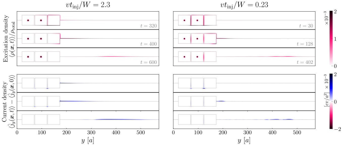
FIG. 12. Three snapshots of the braiding protocol for two values of vt_{\text{inj}}/W (left column and right column). the top panel shows the snapshots in terms of the local excitation density, and the bottom panel shows them in terms of the local current density.
