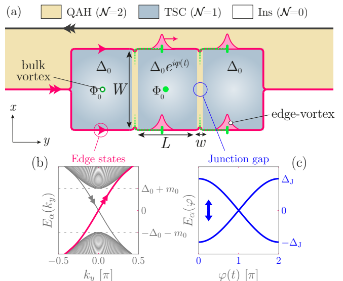
FIG. 2. (a) Full braiding device: two injectors (as in Fig. 1) are used to produce pairs of edge-vortices. The pair of edge-vortices at the back exchanges parity with the bulk vortices upon overtaking a bulk vortex, which is detected by a e/2 charge measurement at the exit. (b) Dispersion of Majorana edge modes (magenta), calculated for an infinite strip of a topological superconductor ( \mathcal{N} = 1 ). (c) Lowest energy levels in an infinite Josephson junction (described in Sec. II) as a function of the superconducting phase. At \phi = \pi these modes become degenerate and correspond to chiral Majorana edge states propagating along the junction [24].
