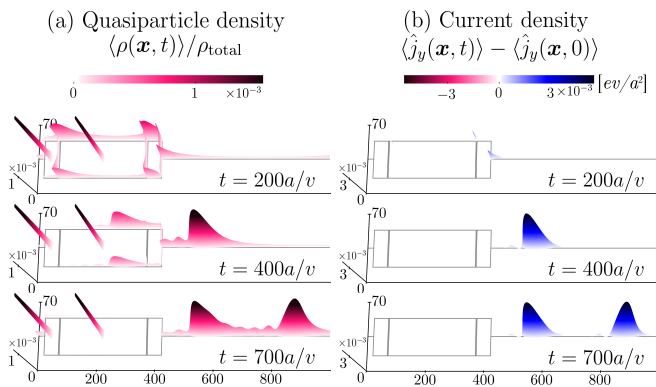
FIG. 3. Time snapshots of a dynamical simulation of the full device during the injection and braiding protocol, (a) Bogoliubov quasiparticle density as defined in equation (4.3) and (b) current density as defined in (3.1). In this simulation vt_{\text{inj}} = 1.5W \ll L , so the edge-vortices injected at the back and front junction are well separated creating two separate e/2 charge pulses upon fusion. An animated version can be found at [25].
