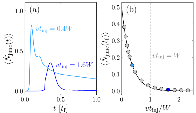
FIG. 9. (a) Quasi-particle number inside the junction as a function of time, for two values of the injection time. (b) Residual quasi-particle number in the junction at some final time t_f = 500a/v as a function of the ratio vt_{\text{inj}}/W . An exponential fit yields \langle \hat{N}_{\text{junc}}(t_f) \rangle = N_0 \cdot \exp(vt_{\text{inj}}/W\beta) with \beta = 0.31 and N_0 = 0.5 .
