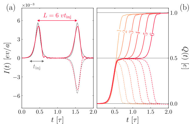
FIG. 4. (a) Simulated (pink) and theoretical (gray) current density at the exit of the superconductor. A system without (with) vortices is represented with dashed (solid) lines. The pulse width t_{\text{inj}} \approx \tau/5.17 is indicated. (b) Corresponding charge increase, for different values of the inter-junction separation L , with values of L/vt shown on top of the curves. All simulations have \tau = 500a/v and W = 42a .
