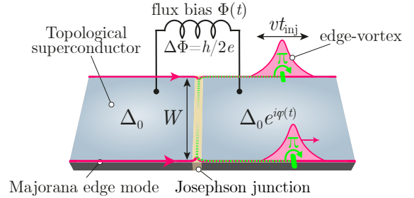
FIG. 1. Edge vortex injector [10], consisting of a Josephson junction in a topological superconductor with co-propagating chiral edge modes. An h/2e flux increment injects a pair of edge-vortices on opposite edges with a protected fermion parity. The corresponding phase domain wall is represented with green lines. The adiabatic description of the injection process assumes that the injection time t_{\text{inj}} = (2\pi\xi_J/W)(d\varphi/dt)^{-1} is long compared to the propagation time W/v along the junction. In this work we relax that assumption, to simulate a device (Fig. 2) where these dynamically injected edge-vortices are braided with Abrikosov bulk vortices.
