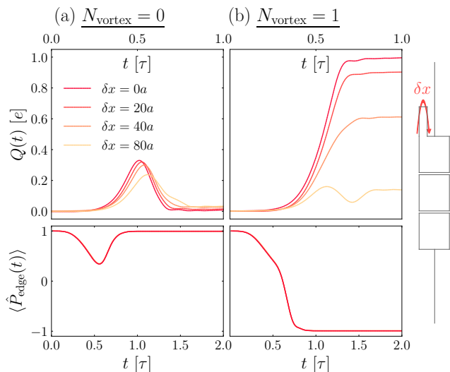
FIG. 6. (Top) Net charge increase at the exit of the superconductors without (a) and with (b) vortices, with four geometrically induced path length differences between the edges \delta x for \tau = 500a/v . (Bottom) Parity of the edge sector for the same data sets. The calculated parity is independent of \delta x . In this case the data sets overlap making the different curves indistinguishable.
