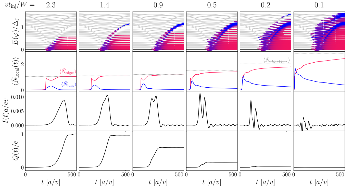
FIG. 13. For different values of vt_{\text{inj}}/W from left to right, (First row) Quasi-particle occupation of the energy levels (thick colored lines). The color of the lines distinguishes between junction (blue) and edge (red) states. (Second row) Quasi-particle number in the junction (blue), edges (red) and their sum at final value (gray dashed line). (Third row) Current at the exit of the superconductor. (Fourth row) Net charge creation at the exit of the superconductor.
