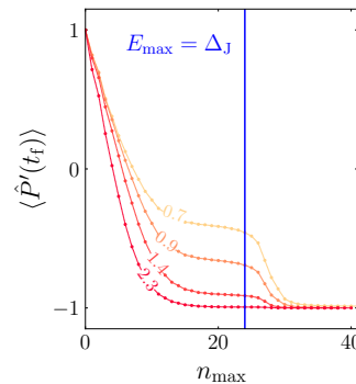
FIG. 11. Convergence of the parity sector \hat{P}' at final time t_f as a function of the index n_{\max} which counts the number of eigenstates included in the calculation. This is done for different values of vt_{\text{inj}}/W which are displayed on the curves. For energies above E_{\max} = \Delta_J , the hybridized edge-junction states are necessary in the convergence of the operator.
