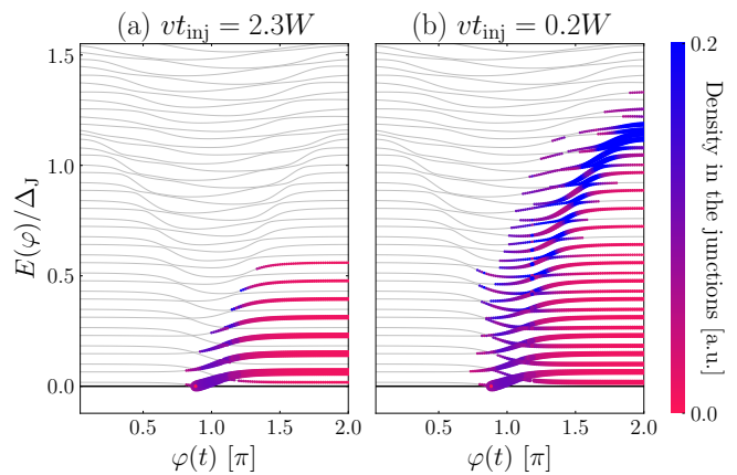
FIG. 7. Quasi-particle occupation of the energy levels (thick colored lines; a thick line signifies a strong occupation) above the ground state level ( E = 0 ), superimposed on the time-independent energy spectrum of H(\varphi) (thin gray lines). The color of the lines distinguishes between junction (blue) and edge (red) states. At fast injection (b), the quasiparticle occupation in the junction levels E_\mu \geq \Delta_J at final time is high. We have removed the vortex state from this figure.
