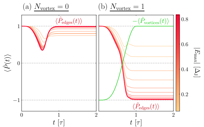
FIG. 5. Evolution of the parity operator expectation value in the initial ground state without (a) and with vortices (b). In panel (b), the parity of the vortices is separated from the edges, and a parity switch is observed. Convergence of the curves as a function of E_{\max} is shown in color.
