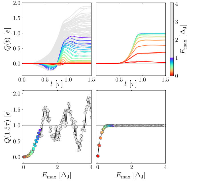
FIG. 10. Convergence of the charge at the exit with two methods (Left) With charge expressed in the local basis using Eq. (A8) where E_{\max} is the maximum energy of the states in the sum over \alpha . (Right) With charge expressed in the basis of eigenstates of H(0) using Eq. (A13) where E_{\max} is the maximum energy of the states in the sums over \alpha, \mu and \nu .
