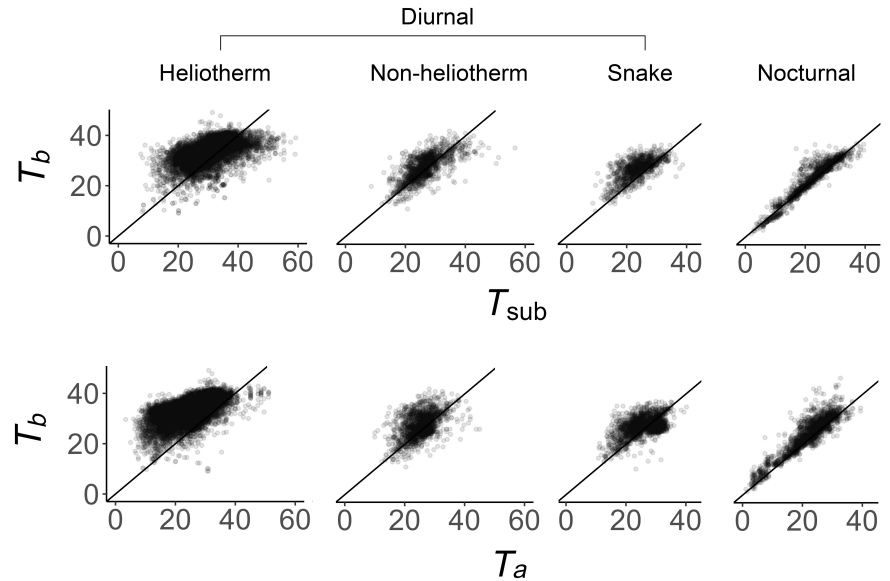
FIGURE 2 Active body temperatures ( T_b ) of the 20,231 individuals used in the analyses, visualized against substrate temperature (top) and air temperatures (bottom). The line represents equality (intercept of 0 and slope of 1). Axis units are degrees Celsius.
