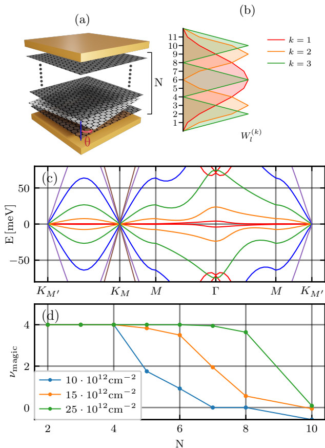
FIG. 1: (a) Device schematics. We consider N -layer graphene with alternating twist angles in a double-gated setup. Here \theta is the physical twist angle. (b) Schematics of layer charge distribution (See Eq. (10)) for N = 11 , showing the three sectors with lowest effective twist angle, k = 1 : red, k = 2 : orange, k = 3 : green. In experiment to date, k = 1 is the flattest, “magic” sector. (c) Single particle band structure for N = 11 . (d) Band filling of the magic sector at different total gate densities. 25 \cdot 10^{12} \text{ cm}^{-2} is the threshold of dielectric breakdown in current hBN-based samples [19].
