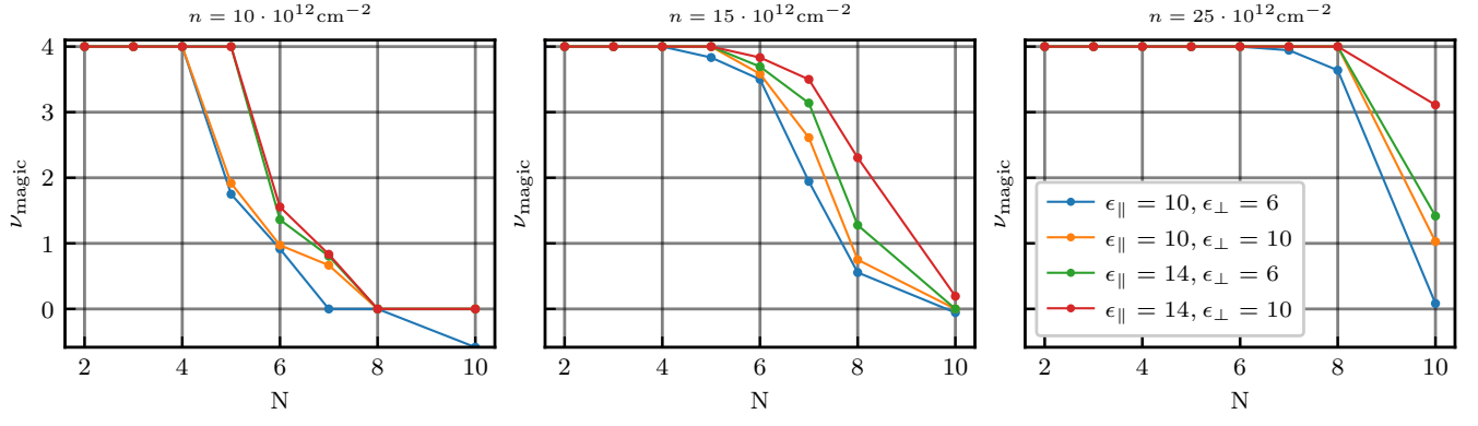
FIG. D4: Dependence of the magic sector filling on interaction strength and the number of layers with gate charge n increasing from left to right. Here we work at zero strain \epsilon_{\text{strain}} = 0.0\% .
