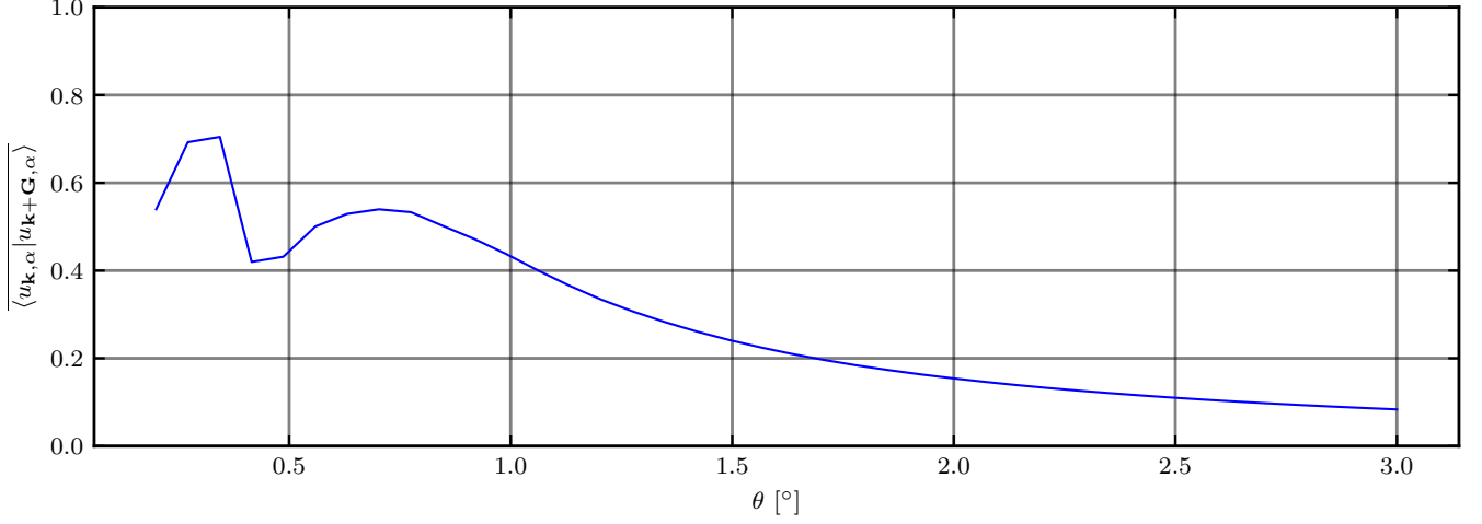
FIG. A1: Dependence of \overline{\langle u_{\mathbf{k},\alpha} | u_{\mathbf{k}+\mathbf{G},\alpha} \rangle} , a quantity that controls the in-plane Hartree correction, on twist angle for N = 2
