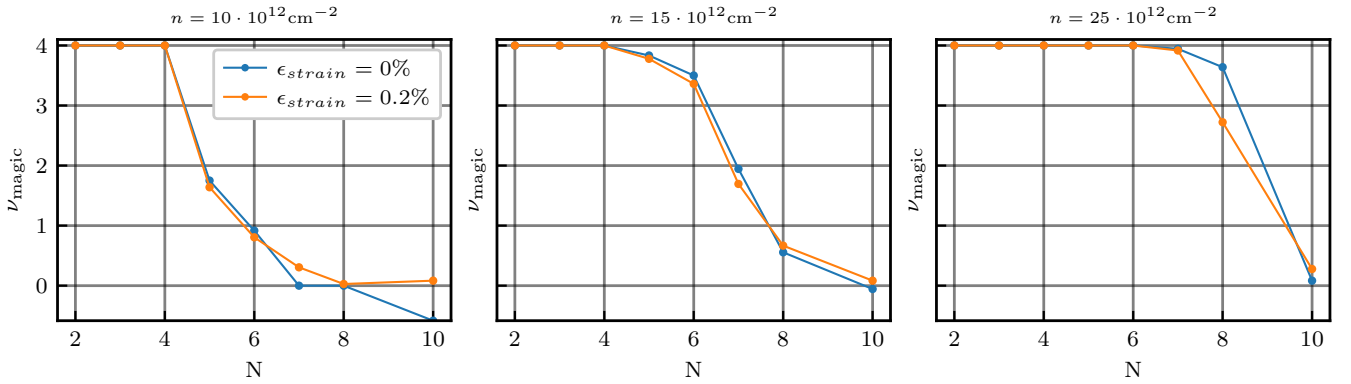
FIG. D3: Strain dependence of charge in the magic sector depending on the gate charge increases from left to right. Here we take \epsilon_{\perp} = 6 , \epsilon_{\parallel} = 10 .
