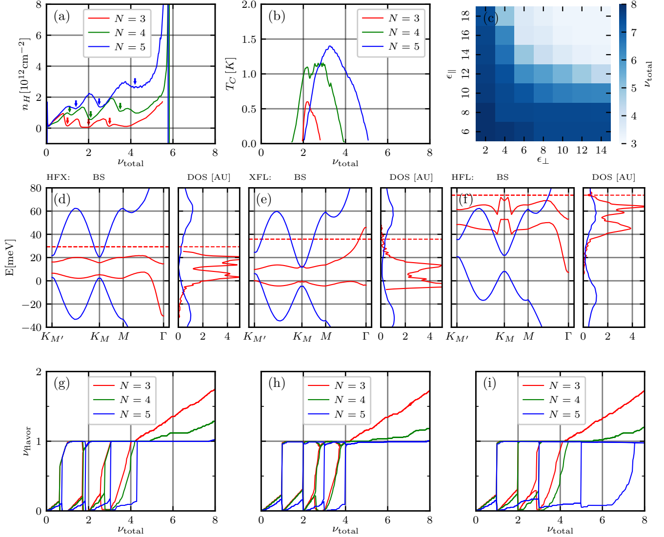
FIG. 2: (a) Experimental data of the Hall density vs. total filling showing the cascade transitions (arrows) for N = 3, 4, 5 , see Ref. [3] for details on the samples and measurements. (b) Corresponding experimental data for T_C domes for N = 3, 4, 5 . (c) Colormap of \nu_{\text{total}} needed to reach filling \nu_{\text{magic}} = 3 of the magic sector in the \varepsilon_{\parallel} - \varepsilon_{\perp} plane. (d) Interacting structures and densities of states for TPG at \nu_{\text{total}} = 4 , including in-plane Hartree and Fock (HFX) terms from Eq. 3. Shown are the k = 1 magic sector (red) and k = 2 nonmagic TBG-like sector (blue). (e) Same as (d) but with layer Hartree potentials and Fock (XFL) (f) Same as (d) but including all terms, that is, HFL. (g) Flavor-resolved magic sector filling showing the cascade with in-plane Hartree and Fock (HFX) for N = 2, 4, 5 . (h) Same as (g), but with out-plane Hartree and Fock (XFL) (i) Same as (g), but including all the terms (HFL).
