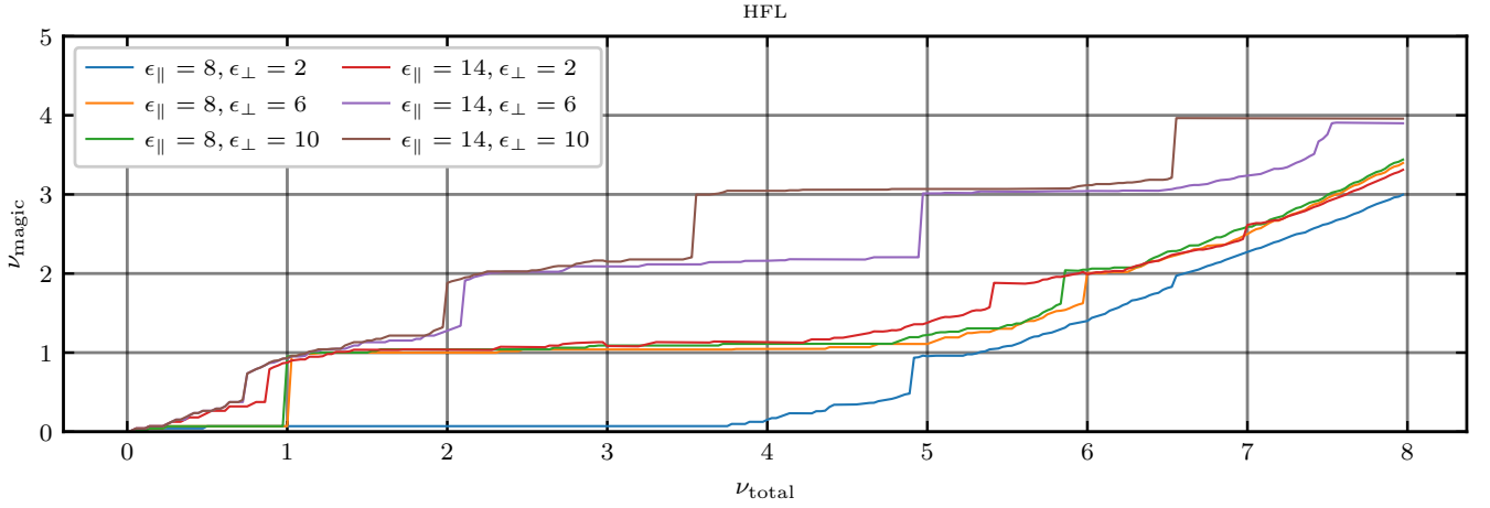
FIG. D2: \nu_{\text{magic}} as a function of \nu_{\text{total}} at different \epsilon_{\perp} and \epsilon_{\parallel} for N = 5 at strain \epsilon_{\text{strain}} = 0.2\% .
