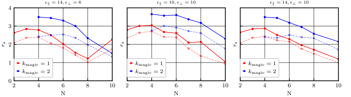
FIG. D6: \varepsilon_{\parallel} and \varepsilon_{\perp} dependence of the r_s plot from the main text.
