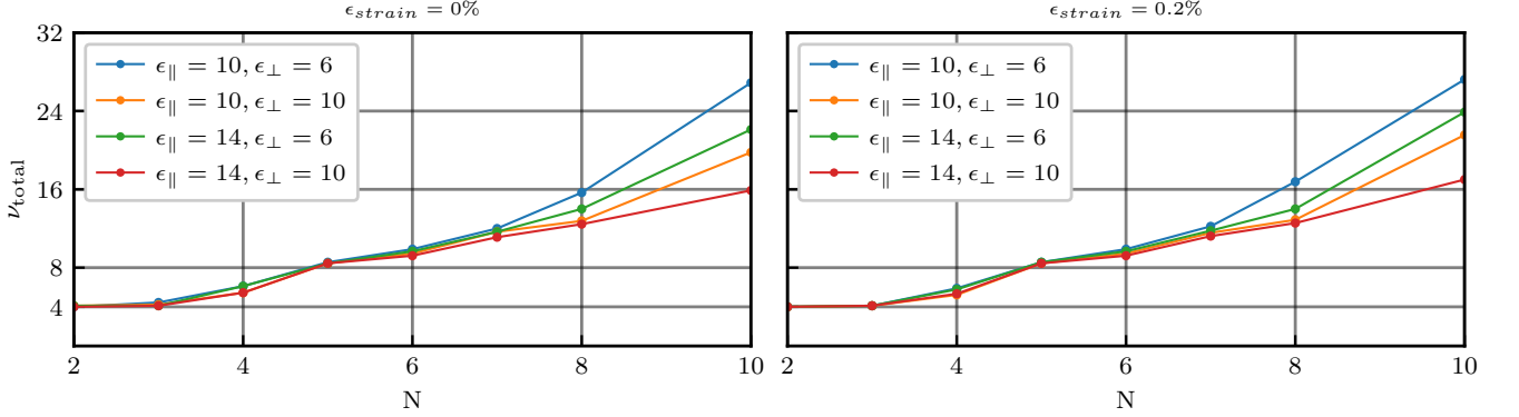
FIG. D5: Interaction strength dependence of total charge needed to fill the magic sector completely. Left: \varepsilon_{\text{strain}} = 0\% . Right: \varepsilon_{\text{strain}} = 0.2\% .
