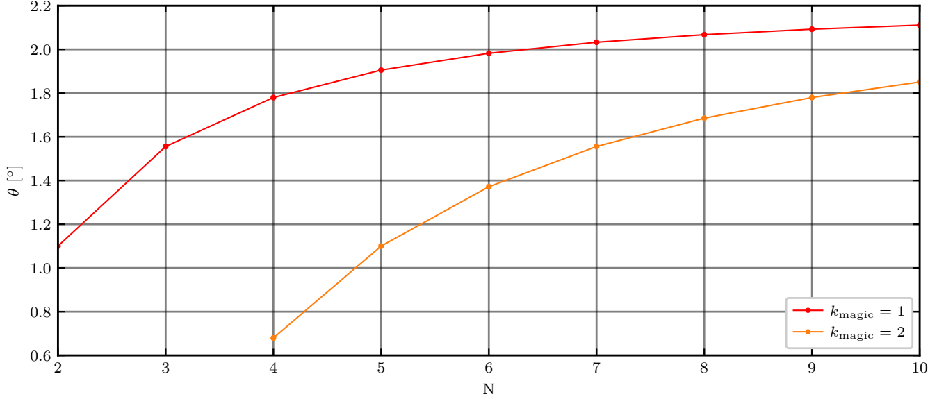
FIG. E1: Physical twist angle for choosing k_{\text{magic}} = 1 (red) or k_{\text{magic}} = 2 (orange) as a function of the layer number N .
