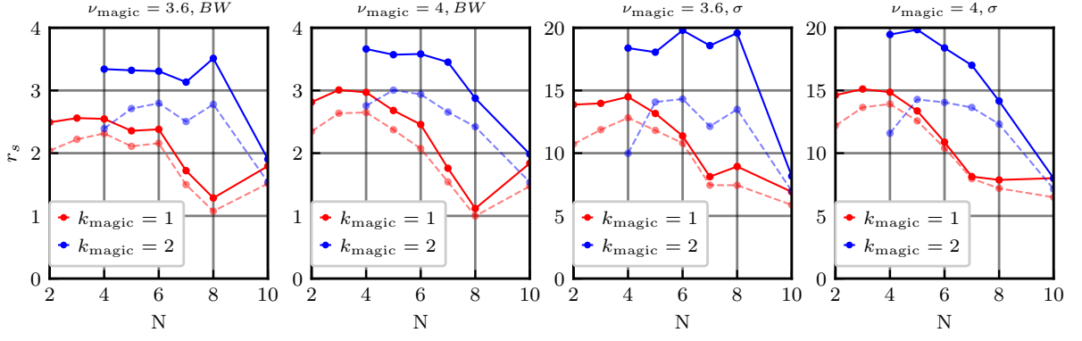
FIG. D7: Dependence of the r_s on working at \nu_{\text{magic}} = 3.6 or \nu_{\text{magic}} = 4 and of using the bandwidth (BW) or standard deviation \sigma as a measure of the width of the active magic bands.
