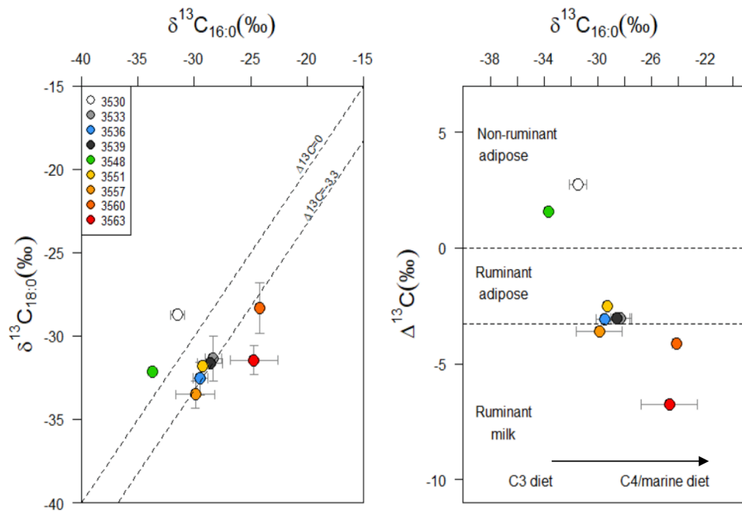
Fig. 7. Stable carbon isotope measurements of C_{16:0} and C_{18:0} fatty acids obtained from our samples of pottery sherds Plot of \delta^{13}C_{16:0} and \delta^{13}C_{18:0} values with SD/2. b Plot of \Delta^{13}C ( \delta^{13}C_{18:0} - \delta^{13}C_{16:0} ) values against \delta^{13}C_{16:0} values with SD/2 obtained from ceramic matrices. NB: We were unable to perform an analysis in triplicate for sample 3542 thus not appearing in the graph (see Table 3 ).
