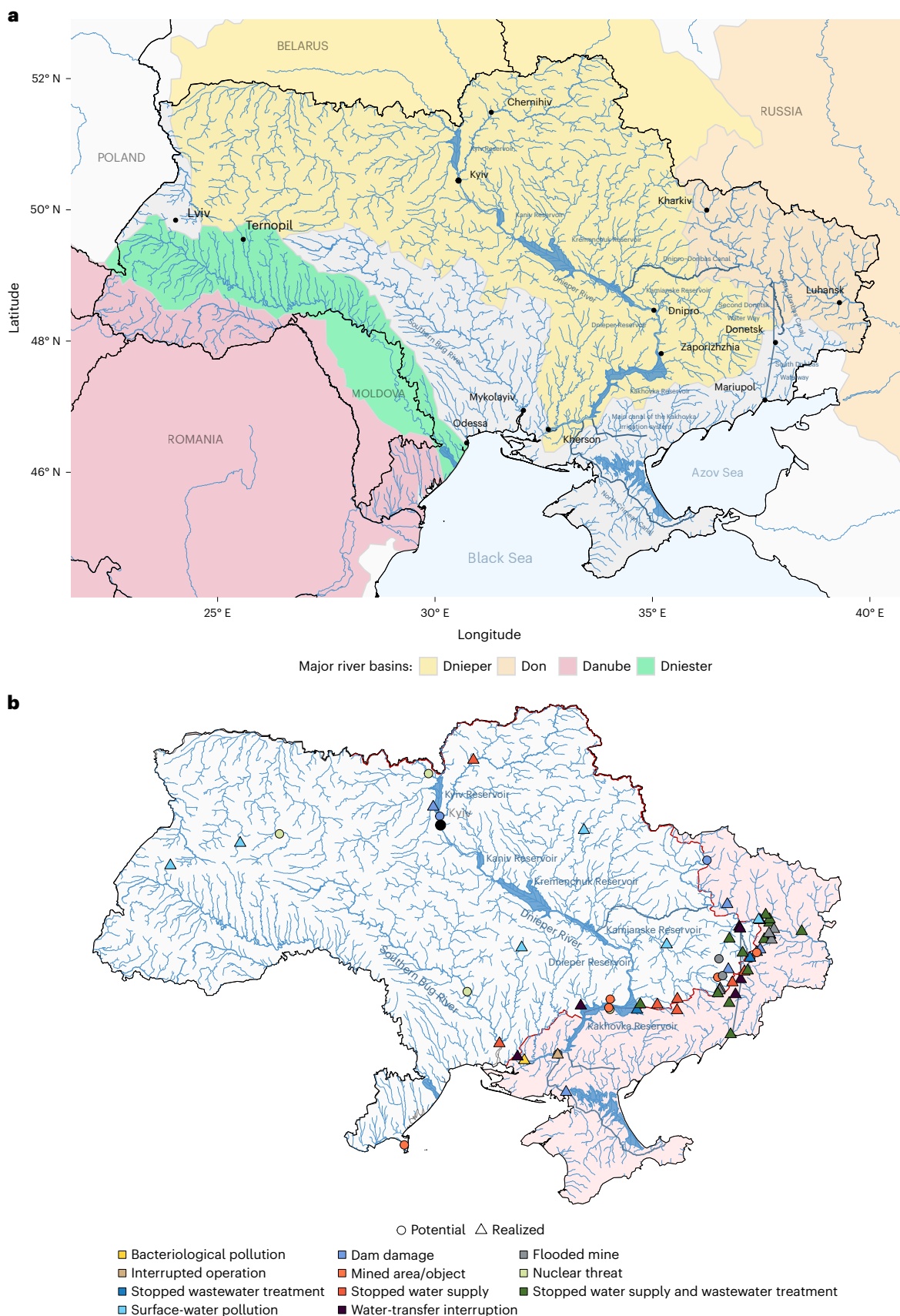
Fig. 2 | The effects of conflict on the water resources and infrastructure in Ukraine. a, Locations of major river basins in Ukraine. b, Identified impacts on water resources and infrastructure in Ukraine (18 February 2022–24 May 2022).
