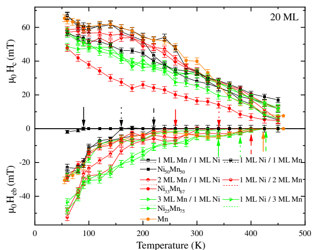
Figure 7. Temperature dependence of the coercivity (positive field axis) and exchange-bias field (negative field axis) of AFM/FM bilayers with 20 ML of pure Mn, \text{Ni}_{25}\text{Mn}_{75} , \text{Ni}_{33}\text{Mn}_{67} , and \text{Ni}_{50}\text{Mn}_{50} -disordered alloys and 3 ML Mn/1 ML Ni, 1 ML Ni/3 ML Mn, 2 ML Mn/1 ML Ni, 1 ML Ni/2 ML Mn, 1 ML Mn/1 ML Ni, and 1 ML Ni/1 ML Mn ALF. The arrows indicate the blocking temperatures for the exchange-bias curves. Arrows with solid lines represent data for disordered alloy samples, arrows with dotted lines represent data for the ALF in which Ni was evaporated first, while arrows with dashed lines represent data for the ALF in which Mn was evaporated first.
