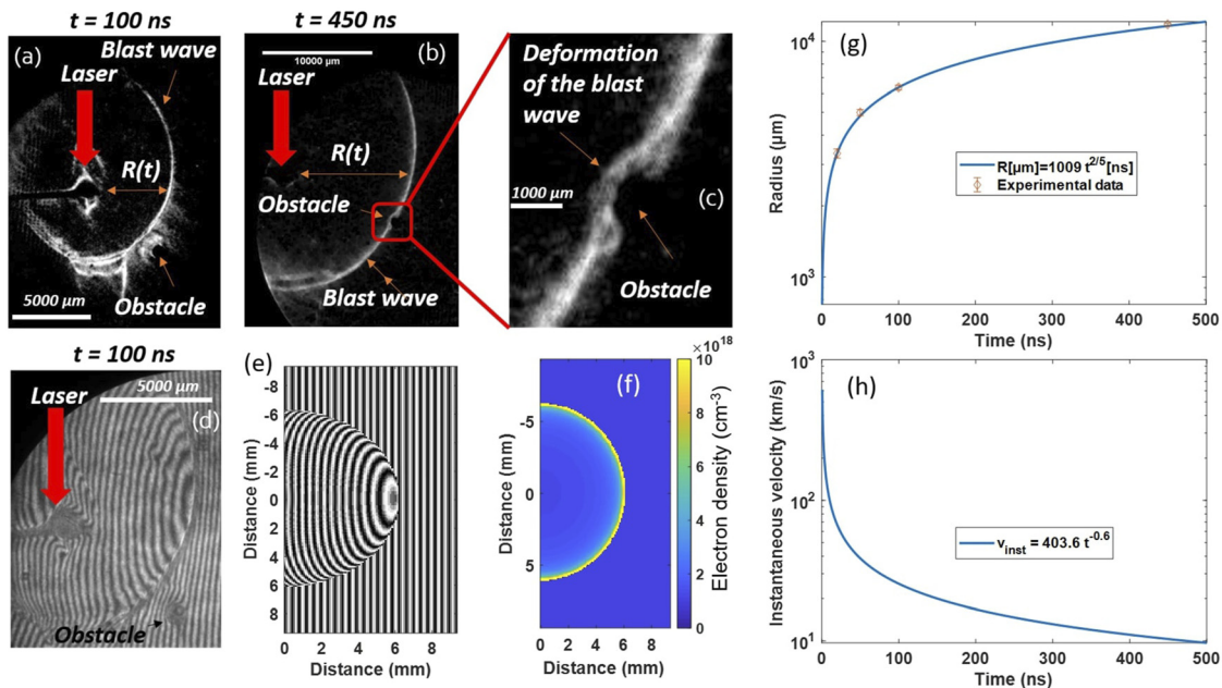
FIG. 3. Experimental results in N_2 at 11.4 mbar. (a) Expansion of a single BW, taken 100 ns after the main pulse, toward the obstacle located 7.07 mm from the carbon rod. (b) Expansion of a single BW, taken at 450 ns, toward the obstacle located 11 mm from the carbon rod. (c) Zoom of (b) showing the deviation of the morphology of the BW from spherical to nonspherical when interacting with the foam ball. (d) Interferogram corresponding to (a). (e) Simulated interferogram. (f) Electron density profile corresponding to (f). (g) Experimental BW radius R vs time taken as illustrated in (a), i.e., parallel to the rod orientation. (h) Instantaneous velocity deduced from radius measurements vs time.
