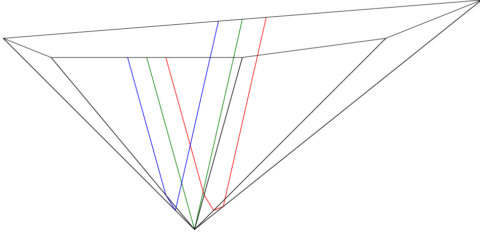
Figure 5.1: An example of toric downgrade: the three-dimensional cone \tau is shown in black, \sigma is green, and the polyhedra \Delta_0 and \Delta_\infty are shown in blue and red.
