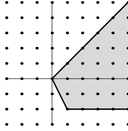
Figure 6.1: An example of a primitive polyhedron.
