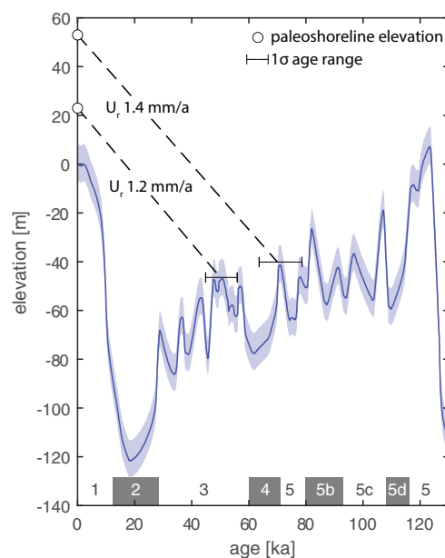
FIGURE 5 Sea-level correlation for the two dated paleoshorelines at the Elafonisi area using the eustatic curve of Lambeck and Chappell (2001). Dashed lines indicate the rock uplift rates based on sea-level highstand correlations. Marine isotope stages are highlighted along the x-axis. [Color figure can be viewed at wileyonlinelibrary.com ]
