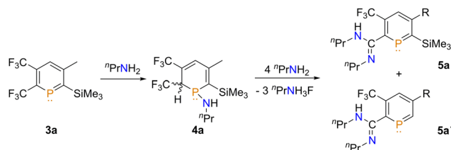
Scheme 2 Reaction of 3a with n PrNH 2 showing the equivalents of amine that has been introduced into the phosphininine. 4a synthesised using 10 equivalents of n PrNH 2 . 5a/a' synthesised using an excess of n PrNH 2 .
