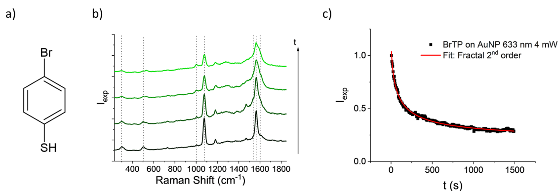
Figure 6. (a) Molecular structure of BrTP. (b) Raman spectra of BrTP on AuNP monolayer after different illumination times (633 nm, 4 mW, 50 \times ). (c) Intensity of a 1076 \text{cm}^{-1} peak is plotted as a function of the illumination time and fitted with a second-order fractal reaction.
