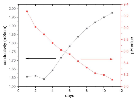
Fig. 6 Long-term investigation of the ionic conductivity and the pH value using an aqueous solution (8.26 mmol L -1 = 14.9 g L -1 ) of the title compound. The lines are only guide for the eyes.
