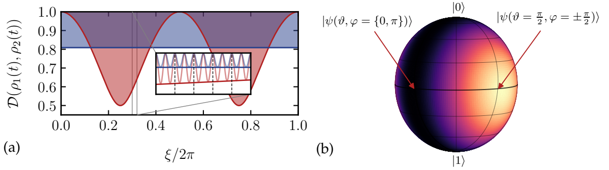
Figure 5.6: (a) Evolution of the trace distance for two different initial state pairs with Rabi angle \phi_2 = 4\pi and a displacement \beta = 0.025 as a function of \xi = -i\alpha t . The state pairs are |\Psi_1\rangle = |\vartheta = 0, \varphi = 0\rangle = |0\rangle (red) and |\Psi_1\rangle = |\vartheta = \frac{\pi}{2}, \varphi = \frac{\pi}{2}\rangle = \frac{1}{\sqrt{2}}(|0\rangle + i|1\rangle) which is an eigenstate of U_{z=2}(t) (blue), paired with the Zeno level |\Psi_2\rangle = |2\rangle . The dark lines show the result of the analytical calculation of the lower envelope, the light, fast oscillating lines show the numerical calculations. The inset shows the fast oscillation of the trace distance due to the Zeno pulse Z_2 acting on |\Psi_2\rangle . The vertical black dashed lines show the positions of the meter's measurement. (b) BLP measure \mathcal{N}_{\text{BLP}} for different initial states |\Psi_1\rangle = |\vartheta, \varphi\rangle on the Bloch sphere spanned by the Zeno subspace \{|0\rangle, |1\rangle\} . The second state of the state pair is the Zeno level |\Psi_2\rangle = |2\rangle outside of this subspace. Yellow indicates the smallest, black the highest value. The parameters are \beta = 0.025 and \phi_2 = 4\pi . The data was obtained numerically but the analytical expression in Eq. (5.50) gives the same results.
