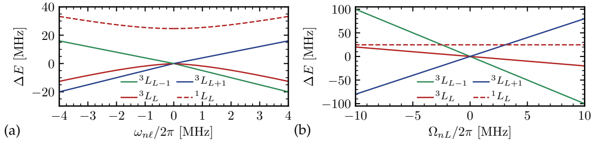
Figure 4.2: Energy shift due to j_1 -coupling as given in Eq. (4.29) (a) and LS-coupling as given in Eq. (4.30) (b) for a g -state. Note that, since the singlets and triplets with J = L mix in (a), the notation ^{2S+1}L_J is not strictly correct any more for \omega_{\ell_1 s_1} \neq 0 and J = L . In both panels, the zero of energy was set to the triplet state for \omega = 0 . The exchange energy was set to 24.665 MHz.
