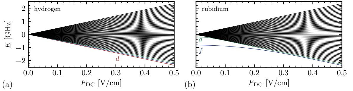
Figure 2.4: Stark map for the n = 51, m = 2 -manifold for hydrogen (a) and rubidium (b). The data was obtained by numerically diagonalising the full Hamiltonian. The states which have \ell = 2 ( d , red), 3 ( f , blue) and 4 ( g , green) at zero field are highlighted in different colours.
