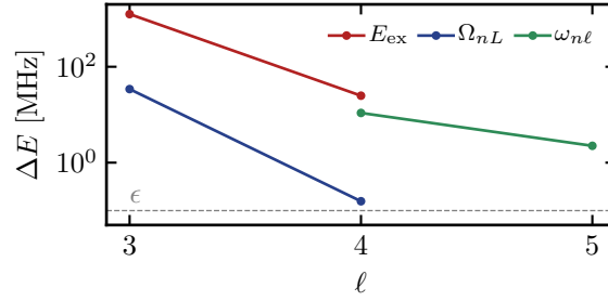
Figure 4.7: Energy shift induced by the exchange energy E_{\text{ex}} , LS-coupling \Omega_{nL} and j_1 -coupling \omega_{nl} of f , g and h states. Missing data points indicate zero energy shifts. The horizontal dashed line indicates the precision of the fit and in the experiment.
