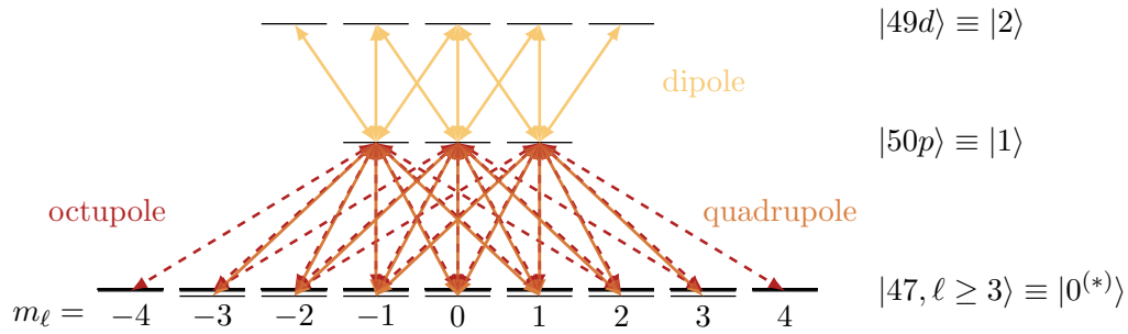
Figure 7.7: Hilbert space of Rydberg atom around 50p which has a dipole allowed transition (yellow) to the 49d state with 18.142 GHz, and quadrupole (orange) and octupole (dashed red) allowed transitions towards the 47\ell manifold. The quadrupole transition couples 50p to the 47f state with a transition frequency of 23.490 GHz, and the octupole couples to 47g with 22.698 GHz.
