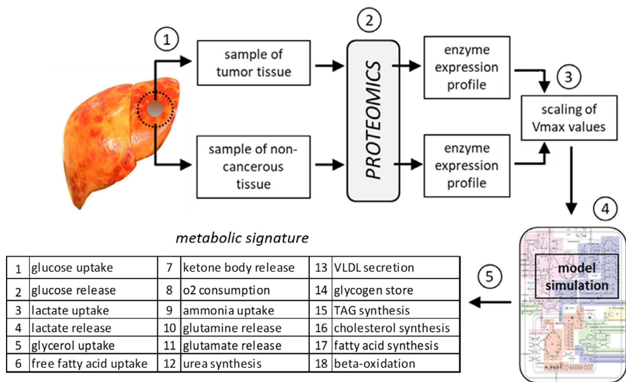
Fig. 7. Main steps in the generation of tumor-specific metabolic signatures. (1) Tissue samples from the tumor (HCC) and the tumor-surrounding noncancerous tissue (control) are taken during curative surgery. (2) Quantitative shotgun proteomics of enzymes and transporters yields protein intensity profiles. (3) Tumor-specific calibration of the kinetic model based on the difference (fold change) between the protein intensity profiles of tumor and control. (4) Model simulations over a 24-h cycle using the plasma profile of exchangeable metabolites and hormones (insulin and glucagon) as model input [17]. (5) 24-h mean values of 21 metabolic functions define the metabolic signature of the tumor.
