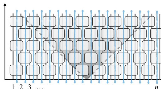
Figure 1. A schematic picture relating the cost of a circuit with the entanglement over cuts for a system of n constituents. The dark grey triangle represents the Lieb-Robinson cone [17–19] that depicts at what rate one expects a linear growth of the entanglement entropy over all cuts in non-equilibrium dynamics generated by a local Hamiltonian.
