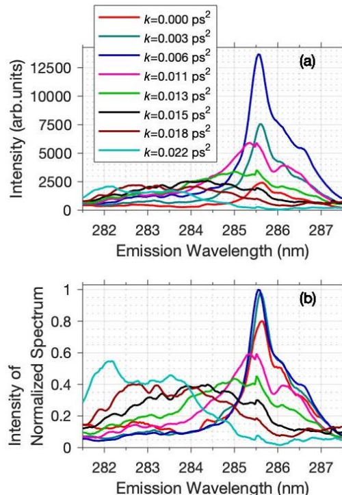
FIG. 3. Examples of experimental UV emission spectra measured following the ultrafast bond-making excitation by linearly chirped femtosecond pulses for different values of the chirp parameter k . Each spectrum corresponds to a cut of the emission map of Fig. 2 at the corresponding chirp. For each emission spectrum, panel (a) presents the measured spectrum and panel (b) the spectral shape obtained by normalizing the measured spectrum by its total intensity. See text for details.
