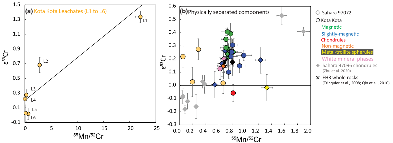
Fig. 3. a) \epsilon^{53}\text{Cr} - ^{55}\text{Mn}/^{52}\text{Cr} isochron diagram for the chemical leachates from Kota Kota. b) Physically separated components from Kota Kota and Sahara 97072 show uncorrelated scatter in the isochron diagram. The lack of correlation could be due to redistribution of Mn during terrestrial weathering or during late parent body processes (e.g., impact heating). The internal errorchron of Kota Kota leachates yields an apparent age of 12.6 Myr after the formation of the solar system (equivalent to an age of 4555 \pm 2 Ma), assuming an initial ^{53}\text{Mn}/^{55}\text{Mn} of 6.28 \times 10^{-6} at 4567 Ma (Trinquier et al., 2008). The relatively young age may reflect local redistribution of sulfide-hosted Mn by impacts or other processes on the parent body of the EH3 chondrites. (Color figure can be viewed at wileyonlinelibrary.com .)
