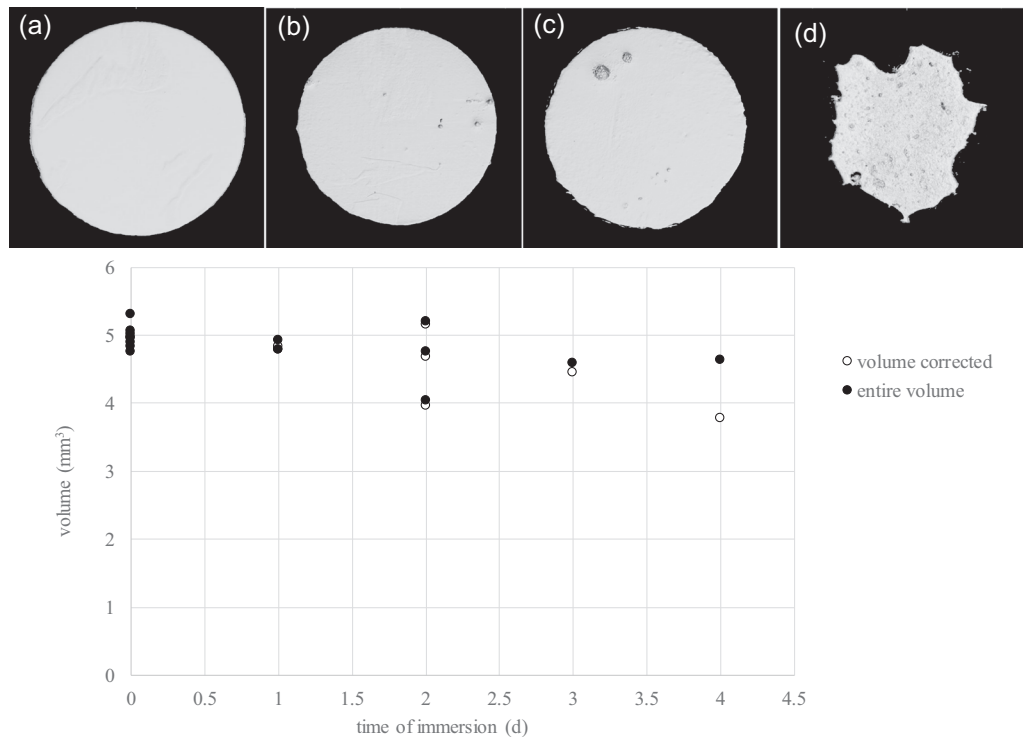
FIGURE 5 Micro-computed tomography (micro-CT) data. Upper level: The depiction of the 3D reconstruction of CT data shows foils having a diameter of (a) 7.9 mm before immersion, (b) 7.8 mm after 1-day immersion time in Dulbecco's modified Eagle's medium (DMEM), (c) 7.8 mm after 4-day immersion time in DMEM, and (d) about 6 mm after 4-day immersion time in corrected simulated body fluid. Lower level: Volume before and after immersion in DMEM shows a decrease with immersion time
