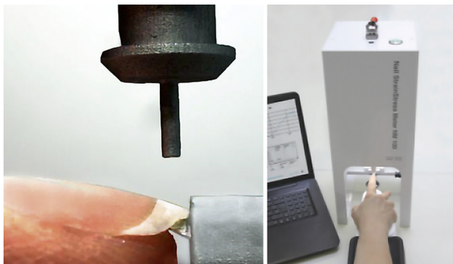
Fig. 4. Operation with the Nail StrainStress Meter NM 100. The nail is placed on the unit's support and a high precision load cell constantly measures the pressure required to clamp down the applicator. The force needed for the deflection of the nail is displayed in real time. When the head touches the surface of the nail, the pressure increases. A force deflection diagram curve is generated from which transversal deformation, slope, resistance to compression, and longitudinal deformation are calculated ( https://www.courage-khazaka.de/images/Downloads/Brochures/Wissenschaftlich/Brochure_NailStrainStressMeter.pdf ; accessed May 7, 2019).
