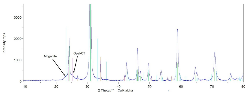
Figure 5. The X-ray diffraction pattern of sample ACu3 (powder sample, background corrected); search-match results in stick patterns: magenta, opal-CT (PDF 00-066-0177); light blue, moganite (PDF 01-073-2991); green, quartz (PDF 01-070-3755); red, calcite (PDF 01-083-0577). The arrows point to the characteristic broad maxima of moganite and opal-CT.
