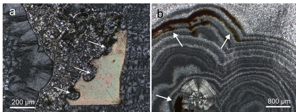
Figure 8. Micrographs in transmitted light (crossed polars) of non-silica phases in the agates from El Picado: (a) calcite grain (sample ACu3), which is partially corroded by SiO 2 (arrows); (b) intercalation of dark banded manganese oxides/hydroxides (sample ACu2) arranged along the chalcedony banding (see arrows) pointing to simultaneous accumulation and precipitation from mineralizing fluids.
