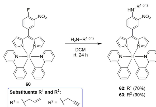
Scheme 4. Nucleophilic substitution of complex 60 with amines.
