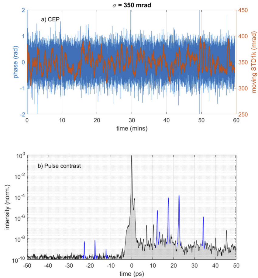
Fig. 7. (a) Carrier envelope phase measurement over a time span of one hour, showing an rms fluctuation of 350 mrad. The orange curve displays rms values calculated on a moving window of 1000 data points. (b) High-dynamic-range measurement of the pulse using a third-order autocorrelator. The three blue peaks before the main pulse are mirror images of those on the trailing side (see text for further details).
