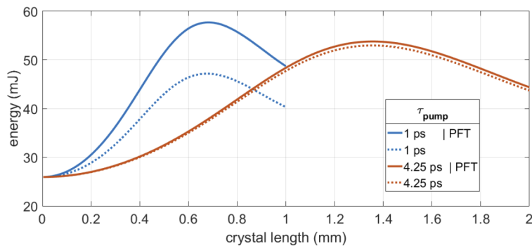
Fig. 5. Simulated pulse energy along the propagation in the OPA crystal for different pump pulse durations and for matched and unmatched pulse front tilt.
