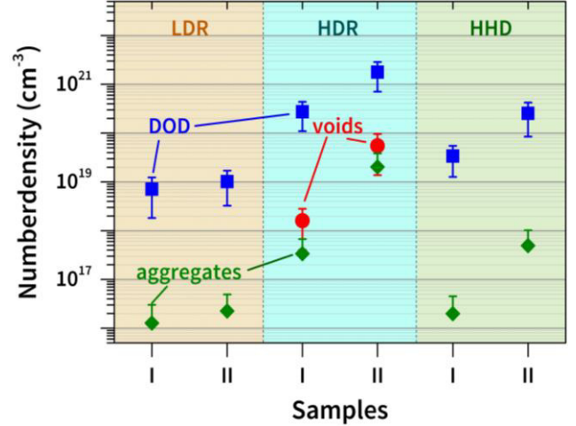
Fig. 3. Number density of DOD, voids, and aggregates in the studied samples. The number density of Si atoms in crystalline silicon is 5 \cdot 10^{22} \text{ cm}^{-3} .
