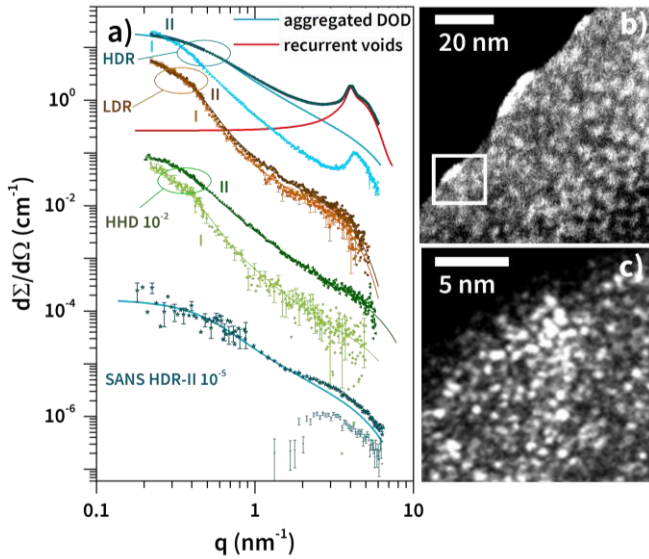
Fig. 1. (a) Experimental SAXS and SANS of the indicated samples and fits according to equations (4) (aggregated DOD) and (8) (recurrent voids) in the SI. The intensities have been shifted vertically by the indicated factors for better visibility. (b) HCDF-TEM and (c) fixed azimuthal HCDF-TEM of sample HDR-II taken in the indicated area in (b).
