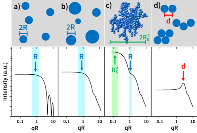
Fig. 2. Model structures and calculated scattering curves of monodisperse particles (a), polydisperse (20 %) particles (b), random aggregated particles (c), and particles clustered with a recurrent distance ( d ) embedded in an amorphous phase. For simplicity, a generalized axes qR is shown.
