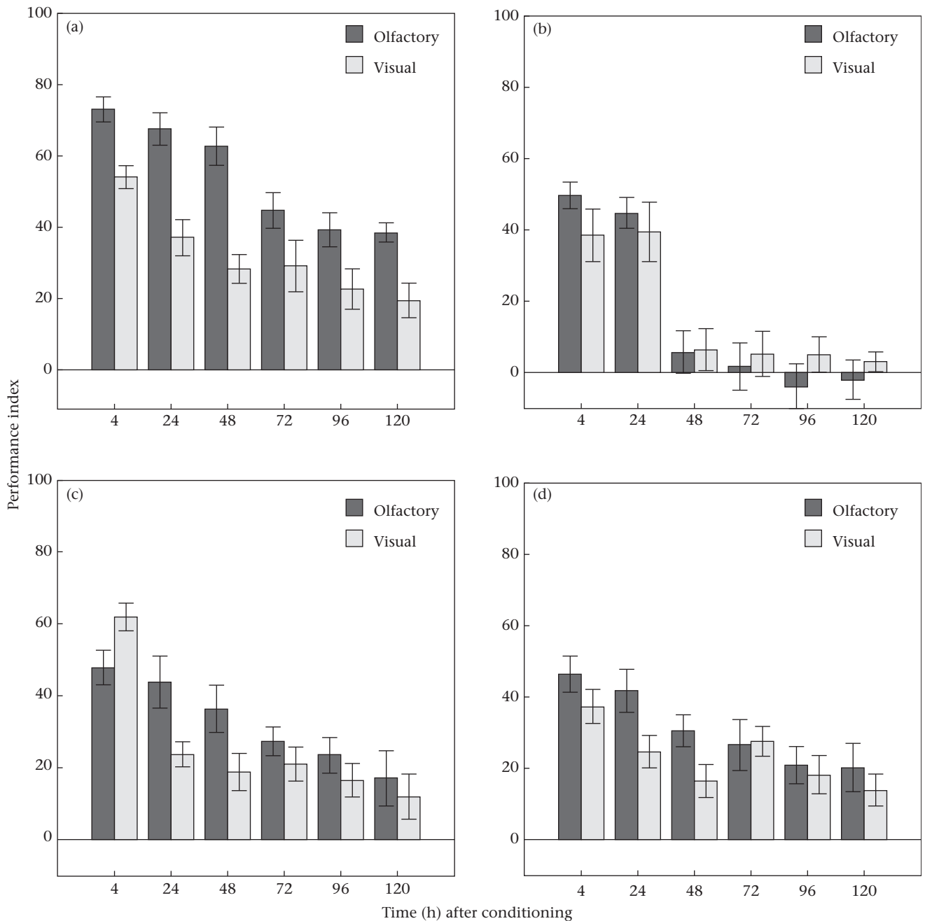
Figure 3. Memory retention expressed as a performance index (PI ± SE) at different time points (4–120 h) for (a) Nv iso , (b) Ng iso , (c) Nv div and (d) Ng div , organized per strain for the response to olfactory and visual learning.
