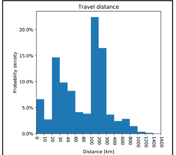
Fig. 2. Simulation of dust transport during field experiment. Probability densities for the height over ground and the distance from the emission source are shown.
