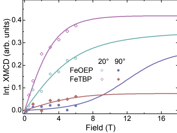
Figure 6: Experimental magnetization curves at 4.5 K of FeOEP and FeTBP (circles and diamonds, respectively) on Au(111) and corresponding spin-Hamiltonian fits (lines).
