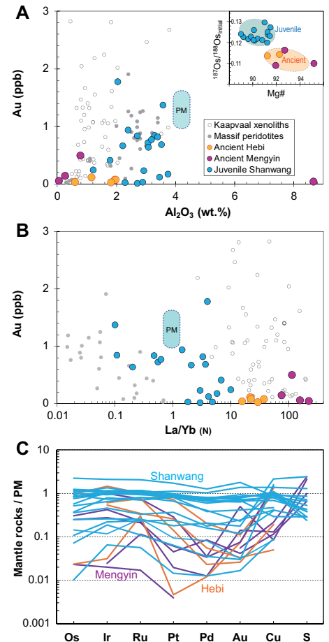
Figure 2. (A–C) Gold and platinum group element (PGE) contents of mantle xenoliths in the North China craton (NCC). Xenoliths in the Hebi and Mengyin areas (A–B) represent relics of Archean to Paleoproterozoic refractory subcratonic lithospheric mantle (SCLM) with later strong metasomatism (Chu et al., 2009; Liu et al., 2011); Shanwang xenoliths are from juvenile SCLM after the destruction of NCC lithosphere (Chu et al., 2009). For many peridotite xenoliths from the Kaapvaal craton, South Africa (Maier et al., 2012), metasomatism contributed abundant sulfur and other volatiles but limited Pd, Au, and Cu to SCLM (C). Data for re-fertilized massif-type peridotites from the Ivrea zone (Italian Alps; Wang et al., 2013) are shown for comparison. Primitive mantle (PM) normalization values are from the literature (McDonough and Sun, 1995; Becker et al., 2006).
