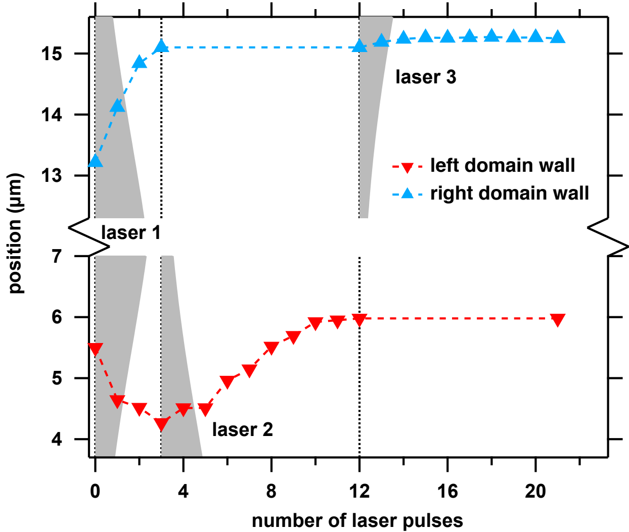
Figure 2. Domain-wall positions of the two domain walls in Fig. 1 along the blue line shown in Fig. 1 (a) as a function of the number of applied laser pulses at laser positions 1 (3 pulses), 2 (9 pulses), and 3 (9 pulses). The respective laser positions are indicated by their gray-shaded Gaussian intensity profiles, plotted onto the vertical dashed lines as zero lines.
