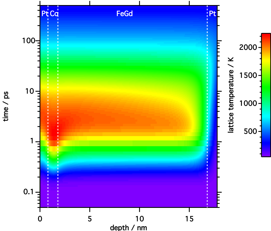
Figure 4. Time dependence of simulated lattice temperature profile along the film depth, for the maximum fluence of 25 \text{ mJ/cm}^2 at the center of the laser spot. Dashed vertical lines mark the positions of the interfaces between the different layers.
