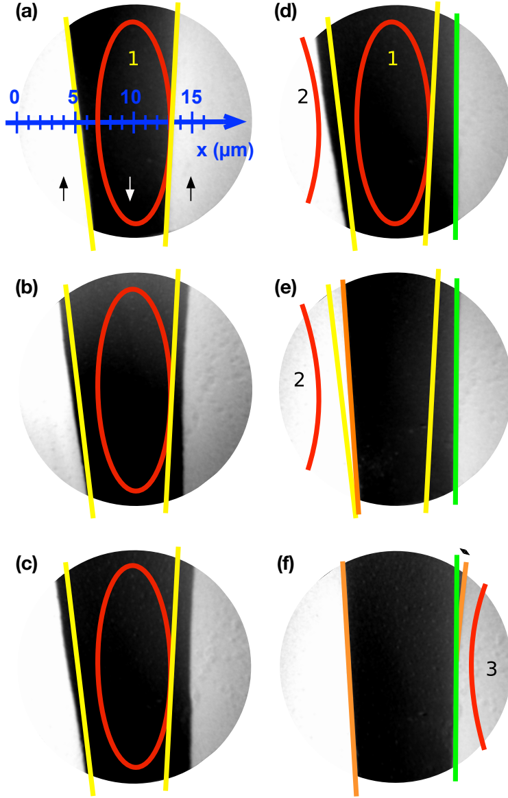
Figure 1. Gd M_5 XMCD-PEEM asymmetry images taken at zero external magnetic field. (a): Starting configuration with two domain walls within the field of view, (b), (c), (d): after first, second, third laser pulse reaching the sample at the red ellipse labeled '1'. (e): Domain image after nine pulses with the laser at the position marked by the ellipse labeled '2', (f): domain image after nine pulses with the laser at position labeled '3'. Yellow, green, and orange lines mark identical positions on the sample surface. The field of view is 20 \mu\text{m} . The blue axis in (a) is used to measure the position of the two domain walls, arrows indicate the local magnetization directions.
