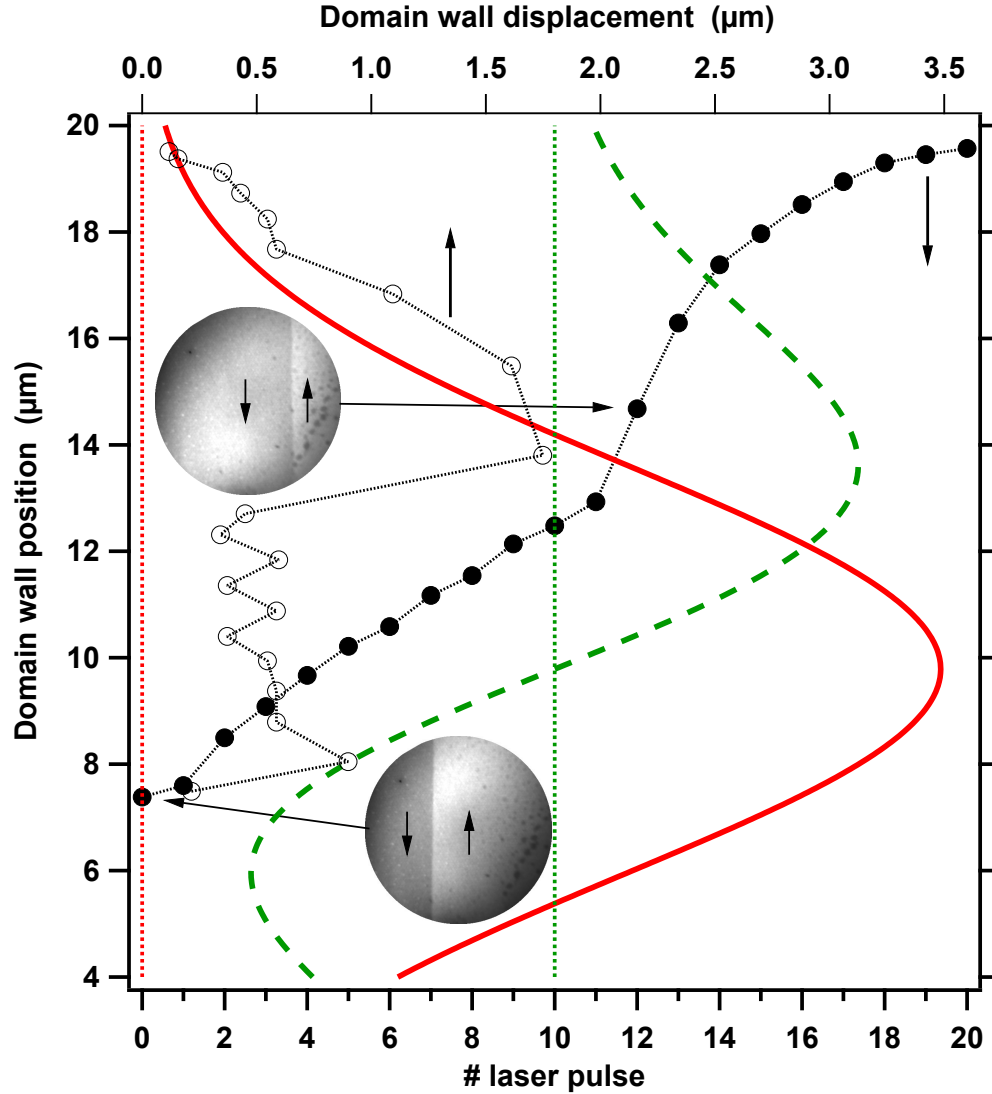
Figure 3. Solid data points: Position of domain wall after application of individual laser pulses (bottom axis) under 1.1 mT constant magnetic field. Open data points: Distance moved by the domain wall (top axis) at each of the laser pulses, plotted versus the position of the domain wall on the left axis. The two insets show the start image and the image after the twelfth laser pulse, taken with positive helicity. Arrows in the insets indicate the local magnetization direction. The external field is pointing downwards in the images. The domain-wall position is measured from left to right along the image horizontal. Red continuous line: Intensity profile of the laser pulse along the same line. Green dashed line: Derivative of the red curve, showing the intensity gradient. The vertical red and green dotted lines are the respective zero lines. The domain wall travels larger distances upon laser pulse excitation when the motion is away from the center of the laser spot and the gradient of the intensity is high.
