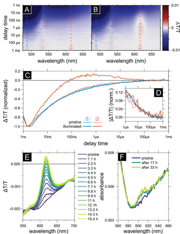
Fig. 1 Effects of prolonged illumination of palladium porphyrin surface-anchored metal–organic frameworks monitored by transient absorption spectroscopy (TAS) and photoluminescence (PL) spectroscopy. (A) TAS data for a pristine PdP SURMOF and (B) a PdP SURMOF after 15.4 hours of photodegradation with a 532 nm pulsed pump laser at 120 \mu\text{J cm}^{-2} (500 Hz repetition rate) under dynamic vacuum ( < 10^{-4} Pa) at room temperature. (C) Normalized TAS kinetic traces integrated over the triplet-dominated region 450–500 nm (1) and the photoproduct-dominated region 605–620 nm (2) for the pristine and illuminated samples from panels (A) and (B). (D) Comparison of the absolute values of the kinetic traces in (C) for delay times > 1 \mu\text{s} . (E) TAS spectra integrated over the time region between 100 ns and 300 ns. The sample was kept under dynamic vacuum ( < 10^{-4} Pa) at room temperature and continuously excited with the pulsed 532 nm pump laser at 120 \mu\text{J cm}^{-2} (500 Hz repetition rate). The shown TAS spectra were taken at a 66 minutes interval. (F) Absorbance spectra of a PdP SURMOF thin film before and after several hours of continuous illumination with a 405 nm CW source at 0.1 \text{ W cm}^{-2} under dynamic vacuum ( < 10^{-4} Pa) at room temperature.
