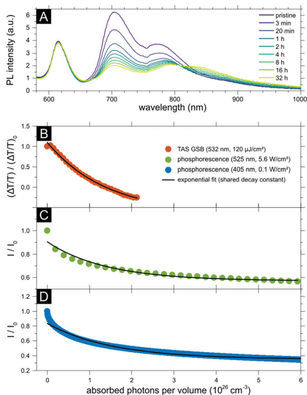
Fig. 2 Changes in PdP SURMOF photoresponse during illumination. (A) PL spectra measured at indicated times during continuous illumination with a 525 nm CW laser at 5.6 \text{ W cm}^{-2} under dynamic vacuum ( <10^{-4} Pa) at room temperature. (B) Relative change in the TAS signal in the GSB region (integrated from 605–620 nm). (C) Relative change in phosphorescence (integrated from 700–720 nm) during illumination with a 525 nm CW laser at 5.6 \text{ W cm}^{-2} at room temperature under dynamic vacuum ( <10^{-4} mbar). The horizontal axis range of 6 \times 10^{26} \text{ cm}^{-3} corresponds to 30 minutes of illumination. (D) Relative change in phosphorescence (integrated from 700–720 nm) during illumination with a 405 nm CW laser at 0.1 \text{ W cm}^{-2} at room temperature under dynamic vacuum ( <10^{-4} mbar). The horizontal axis range of 6 \times 10^{26} \text{ cm}^{-3} corresponds to 22 hours of illumination. The black line represents a mono-exponential fit as a guide to the eye, the decay constant being 1.5 \times 10^{26} \text{ cm}^{-3} for all three panels.
