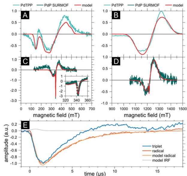
Fig. 3 PdTPP EPR spectra in the X-band (A) and Q-band (B), PdP SURMOF EPR spectra in the X-band (C) and Q-band (D). The samples were measured at 20 K with 532 nm photoexcitation. Simulated model spectra are shown in red. Measured spectra were derived by integrating the first 500 ns of data after the laser flash, then normalizing to unity. Simulations were performed as described in the text, with the fitting parameters given in Table 1. (E) X-band measurement of photoreacted PdP SURMOF, normalized transients for the radical pair and the emissive portion of the triplet signal, with the radical pair decay modelled as a first-order exponential convolved with a Gaussian instrument response function, shown in grey. Transients crossing the zero-line suggest driving by the microwave field and suggest that the true lifetimes are longer than those indicated here.
