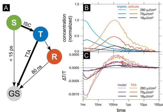
Fig. 5 Model of PdP SURMOF photoresponse. (A) Schematic model showing how excited states can move between singlet (S) and triplet (T) exciton states, radical pair states (R) and the ground state (GS). (B) Model of the radical pair population dynamics. The triplet population is taken directly from TAS and not modelled. The populations are normalized to the maximum of the highest excitation fluence kinetic (280 \mu J cm -2 ). (C) Comparison of modelled and experimental TAS kinetics in the GSB-dominated wavelength region 605–620 nm.
