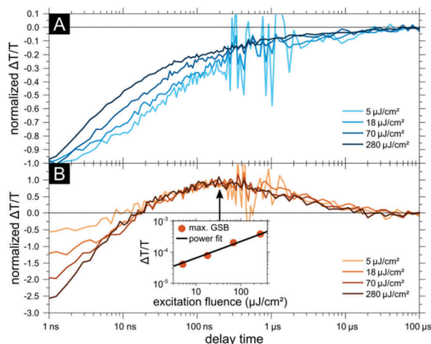
Fig. 4 Excitation fluence dependence of transient absorption measurements under dynamic vacuum ( < 10^{-4} Pa) at room temperature. (A) Integrated triplet PIA kinetics (450–500 nm) show a strong fluence-dependence. (B) In contrast, the decay of the integrated charge-induced GSB kinetics (605–620 nm) does not change with varying excitation intensities. The inset shows how the radical GSB maximum signal (at around 200 ns) scales with excitation fluence. The maximum follows a power law with an exponent of 0.5 (black line).
