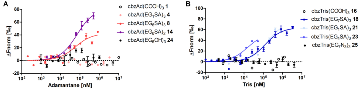
Figure 2. Microscale thermophoresis measurements with intact R18 labeled X31 virus against a) different adamantane-based or b) Tris-based constructs. The change in fluorescence intensity during thermophoresis is shown as a function of the construct's concentration. Data points are one-sited fit. Error bars indicate the SEM ( N \geq 4 ).
