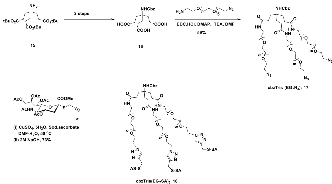
Scheme 4. Synthesis of Tris core trivalent sialoside with EG 7 spacer.
