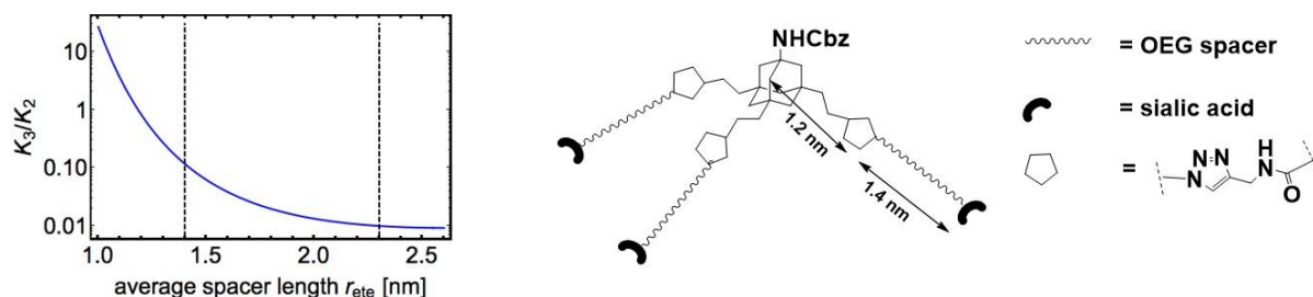
Figure 3. Trivalent vs. divalent binding: The ratio of the trivalent dissociation constant K_3 and the divalent dissociation constant K_2 , according to Eq. 2. The distance between 1.4 nm and 2.3 nm that has to be bridged by the inhibitor spacer to reach HA binding pocket, is indicated by a dashed vertical line.
