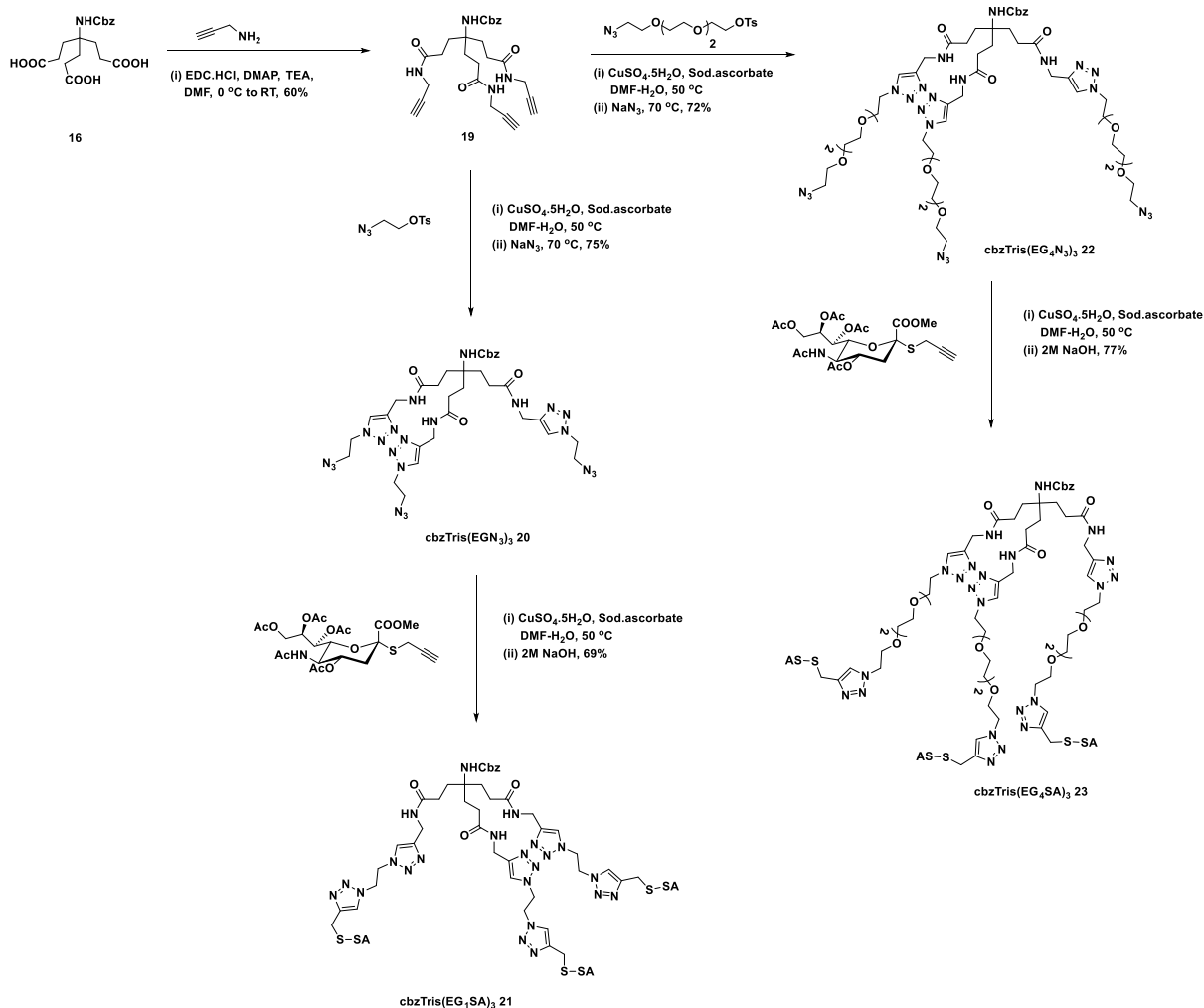
Scheme 5. Synthesis of Tris core trivalent sialosides with an EG 1 and EG 4 spacer.
