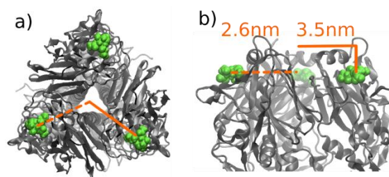
Figure 1. a) Top and b) side view of the HA -region (pdb: 1hgg). Bound sialic acid is highlighted in green.
