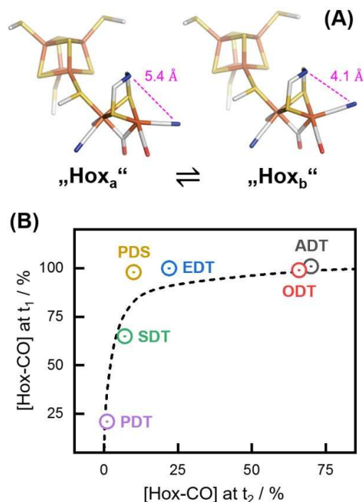
Figure 4. Conceivable isomers of Hox and simulation of relative Hox-CO populations. (A)
