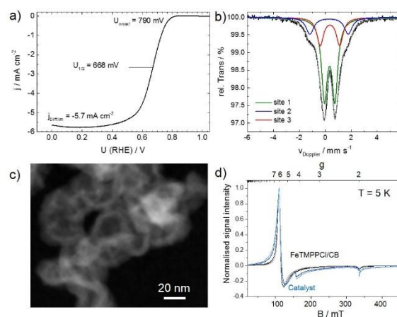
Figure 1. a) RDE measurement of our catalyst in 0.1M H 2 SO 4 , b) room temperature Mössbauer spectrum, c) STEM image and d) X-band EPR spectrum of the catalyst (5 K). For reasons of comparison the FeTMPPCI/CB precursor spectrum is added in d).
