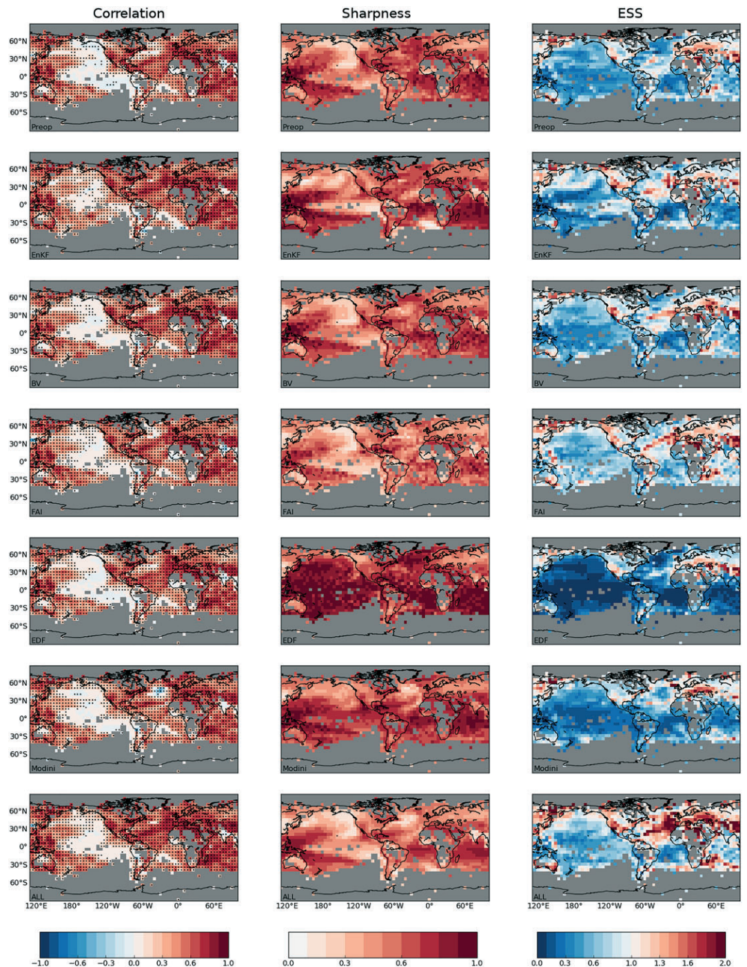
Figure 9. Correlation ( r_{HO} \times |r_{HO}| ; first column) and sharpness ( p , second column) according to the decomposition of ESS (third column) for standardized surface air temperature at lead years 2–5 from Preop-LR and the test-suite experiments. Skill is assessed w.r.t. HadCRUT4 for hindcasts initialized from 1960 to 2011. Stippling on correlation patterns indicates statistical significance at the 95% confidence level. ESS = ensemble spread score; Preop = preoperational MiKlip prediction system; EnKF = ensemble Kalman filter; BV = bred vector; FAI = filtered anomaly initialization; EDF = ensemble dispersion filter.
