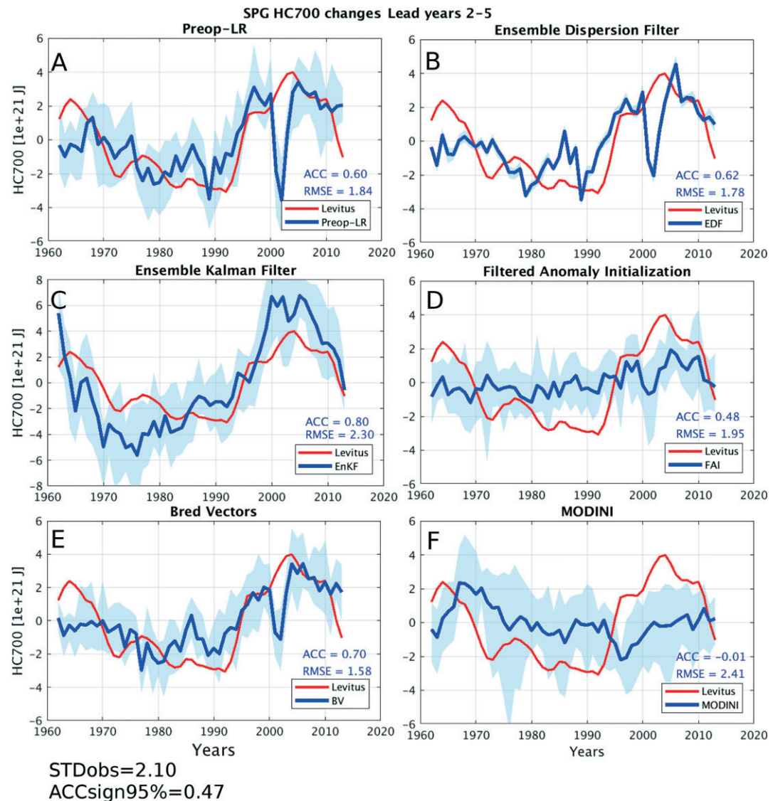
Figure 7. Time series of the North Atlantic SPG HC700 ( 1e+21 J) from NOAA/NODC (red) and the initialized hindcasts at lead years 2–5 (blue). In bold solid is the ensemble mean and shading indicates the range of the ensemble members. ACC is the anomaly correlation coefficient and RMSE is the root mean squared error for the ensemble mean initialized hindcasts started over the period 1960–2011. The 4-year running mean is applied to the NOAA/NODC data. STDobs represents variability in the observational correlation data set. ACCsign95% gives a threshold for significant correlation coefficients; it is estimated using the t test at 5% level, using the autocorrelation of the time series to estimate the degrees of freedom. SPG = subpolar gyre; Preop-LR = preoperational MiKlip prediction system in low-resolution configuration; HC700 = ocean heat content in the upper 700 m.
