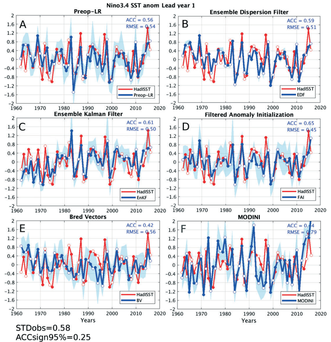
Figure 4. Time series of SST anomalies ( ^{\circ}\text{C} ) averaged over the Nino 3.4 region ( 5^{\circ}\text{S} – 5^{\circ}\text{N} and 170 – 120^{\circ}\text{W} ) from HadISST1.1 (red) and the ensemble mean hindcasts at lead year 1 (blue). Shaded is the range between the minimum and maximum ensemble members. Empty (filled) circles indicate even (odd) years. ACC is the anomaly correlation coefficient and RMSE is the root mean squared error for the ensemble mean hindcasts which are initialized over the period 1961–2015. STDobs represents variability in the observational data set (in ^{\circ}\text{C} ). ACCsign95% gives a threshold for significant correlation coefficients. It is assessed using the t test at 5% level, using the autocorrelation of the time series to estimate the degrees of freedom. SST = sea surface temperature; Preop-LR = preoperational MiKlip prediction system in low-resolution configuration.
