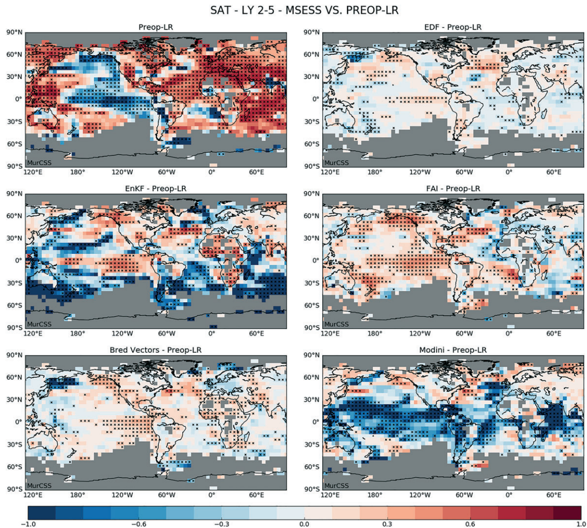
Figure 2. MSESS for SAT w.r.t. the HadCRUT4 climatology for lead years 2–5 from Preop-LR (top left panel). MSESS for SAT w.r.t. Preop-LR for the test-suite experiments (first to third rows). Hindcasts initialized from 1960 to 2011 are evaluated. The range of MSESS is from -\infty to +1. Stippling indicates significant MSESS values as estimated with the bootstrap method at the 95% confidence level. SAT = surface air temperature; Preop-LR = preoperational MiKlip prediction system in low-resolution configuration; EDF = ensemble dispersion filter; EnKF = ensemble Kalman filter; FAI = filtered anomaly initialization; MSESS = mean squared error skill score.
