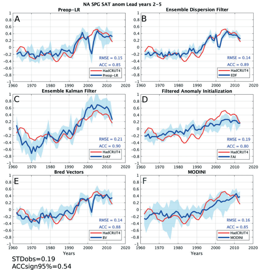
Figure 6. Same as in Figure 4 for the North Atlantic SPG SAT in degrees Celsius from HadCRUT4 (red) and the ensemble mean hindcasts at lead years 2–5 (blue) initialized over the period 1960–2011. The 4-year running mean is applied to the HadCRUT4 data. Preop-LR = preoperational MiKlip prediction system in low-resolution configuration; SPG = subpolar gyre; SAT = surface air temperature.
