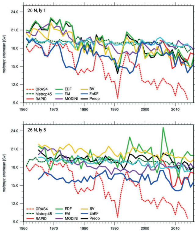
Figure 8. The time series of the Atlantic meridional overturning circulation (in Sv) at 26.5° N latitude 1,000-m depth from the initialized hindcasts (Preop-LR = black, the EnKF = blue, the BV = yellow, FAI = cyan, MODINI = magenta, and the EDF = green) in the first (upper panel) and fifth (lower panel) lead years and the uninitialized historical simulation (green dashed), the ORAS4 reanalysis (red dashed), and the RAPID observations (red solid). EDF = ensemble dispersion filter; FAI = filtered anomaly initialization; BV = bred vector; EnKF = ensemble Kalman filter; Preop = preoperational MiKlip prediction system.
