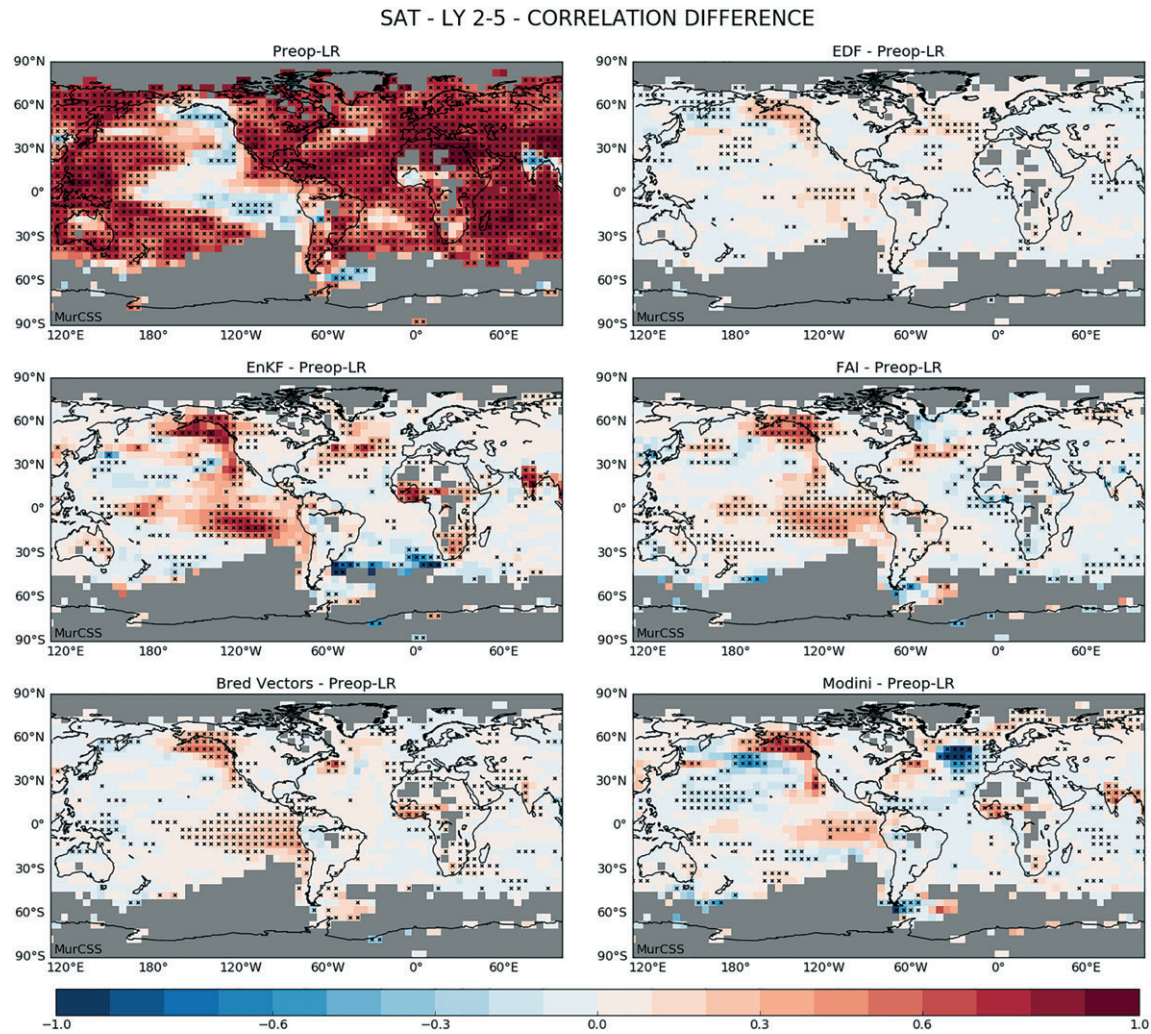
Figure 1. Correlation skill for SAT w.r.t. HadCRUT4 for lead years 2–5 from Preop-LR (top left panel) and the correlation skill difference between a particular test-suite experiment and Preop-LR (first to third rows). Hindcasts initialized from 1960 to 2011 are evaluated. Stippling indicates statistical significance estimated with the bootstrap method that the value is positive at the 95% confidence level. Areas are masked where time series from the observational data set contain missing values. SAT = surface air temperature; Preop-LR = preoperational MiKlip prediction system in low-resolution configuration; EDF = ensemble dispersion filter; EnKF = ensemble Kalman filter; FAI = filtered anomaly initialization.
