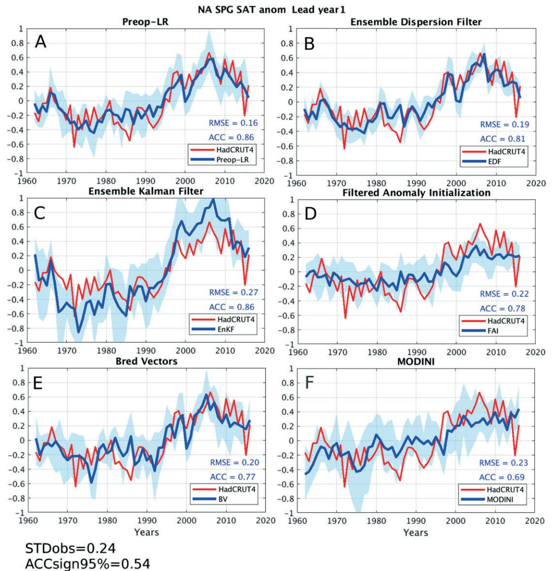
Figure 5. Same as in Figure 4 for the North Atlantic subpolar gyre (SPG) SAT in degrees Celsius ( 50^{\circ} – 60^{\circ} N and 65^{\circ} W– 10^{\circ} E) from HadCRUT4 (red) and the ensemble mean hindcasts at lead year 1 (blue) initialized over the period 1961–2015. SAT = surface air temperature; Preop-LR = preoperational MiKlip prediction system in low-resolution configuration.
