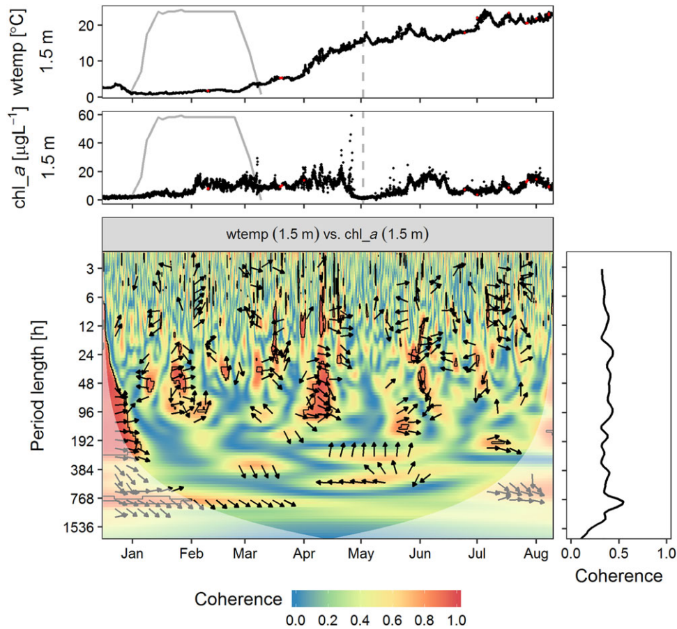
Fig. 4. Upper panels: Time series of water temperature (wttemp) ( ^{\circ}\text{C} ) and Chl a ( \mu\text{g L}^{-1} ) measured hourly at a depth of 1.5 m in the Müggelsee; time window with an ice cover (gray line); onset of the clear water phase (vertical dashed line). Bottom panel: Wavelet coherence between wttemp and Chl a ; black lines, arrows and lighter shade as in Fig. 3; \gamma -axis log 2 -transformed. Right margin panel: Global wavelet coherence, calculated as the arithmetic mean over time.
