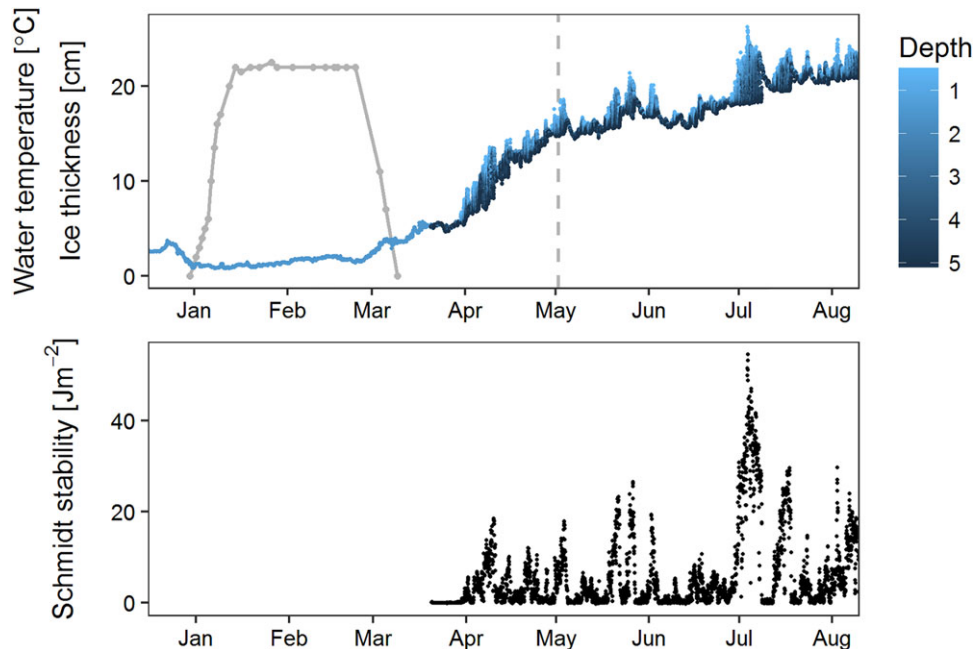
Fig. 2. Upper panel: Time series of water temperature ( ^{\circ}\text{C} ) in the Müggelsee with blue color gradient according to measurement depth; ice thickness (cm) (gray dots and line); peak of zooplankton abundance as an indicator of the clear water phase, calculated as the local maximum of the fit of a Weibull function to weekly cladocera abundance data (Rolinski et al. 2007; vertical dashed line). Bottom panel: Time series of Schmidt stability ( \text{J m}^{-2} ), calculated from vertical water temperature profiles.
