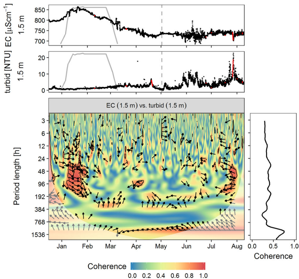
Fig. 7. Upper panels: Time series of electrical conductivity (EC) ( \mu\text{S cm}^{-1} ) and turbidity (turbid) (NTU) measured hourly at a depth of 1.5 m in the Müggelsee; time window with an ice cover (gray line); onset of the clear water phase (vertical dashed line). Bottom panel: Wavelet coherence between EC and turbid; black lines, arrows, and lighter shade as in Fig. 3; \gamma -axis \log_2 -transformed. Right margin panel: Global wavelet coherence, calculated as the arithmetic mean over time.
