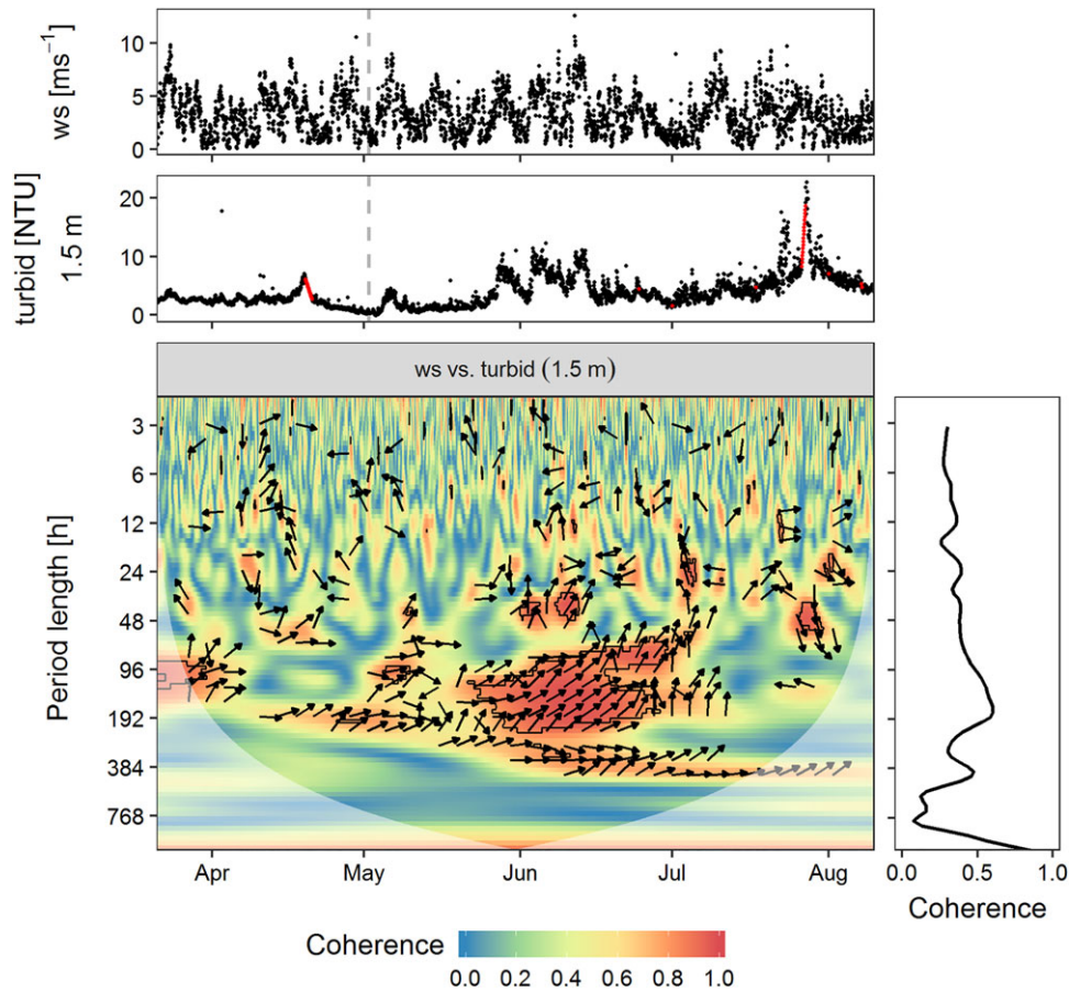
Fig. 8. Upper panels: Time series of wind speed ( ws ) ( m\ s^{-1} ) measured hourly at a height of 4 m above the Müggelsee and turbidity ( turbid ) (NTU) measured hourly at a depth of 1.5 m in the Müggelsee; time window with an ice cover (gray line); onset of the clear water phase (vertical dashed line). Bottom panel: Wavelet coherence between ws and turbid ; black lines, arrows, and lighter shade as in Fig. 3; y -axis \log_2 -transformed. Right margin panel: Global wavelet coherence, calculated as the arithmetic mean over time.
