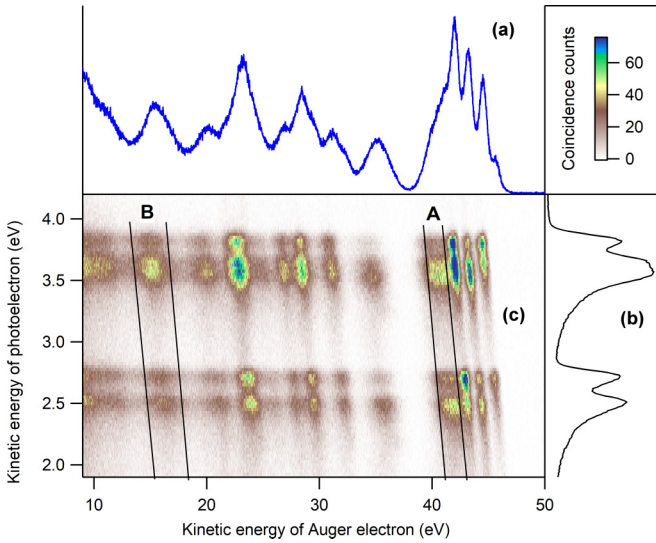
FIG. 1. Energy correlation between photoelectrons and Auger electrons, measured at a photon energy of h\nu = 81 eV. Panel (c) displays the two-dimensional coincidence map between the 3d^{-1} photoelectrons and the Auger electrons. Panels (a) on the top and (b) on the right side show the resulting Auger-electron and 3d^{-1} photoelectron spectra, respectively. The diagonal lines show the different \text{HBr}^{2+} final states, and zones A and B indicate the final states selected for the PCI analysis presented in Fig. 2.
