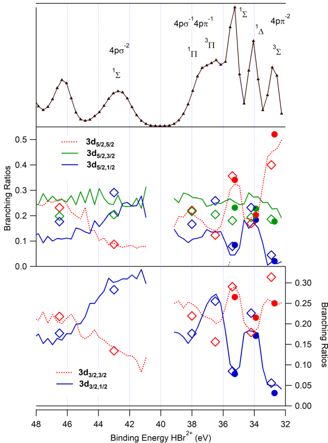
FIG. 5. The lower and the middle panels show the branching ratios for the population of the \text{HBr}^{2+} states via the decays of the different 3d_{3/2}^{-1} and 3d_{5/2}^{-1} components, respectively. The lines are obtained from the fit analysis of the diagonal lines in Fig. 1(c) (see text). The solid dots represent experimental values of Ref. [18] and the open squares represent those of the present calculation. The top panel is a detail of Fig. 3 and represents the population of the \text{HBr}^{2+} final states by the 3d^{-1} Auger decay.
