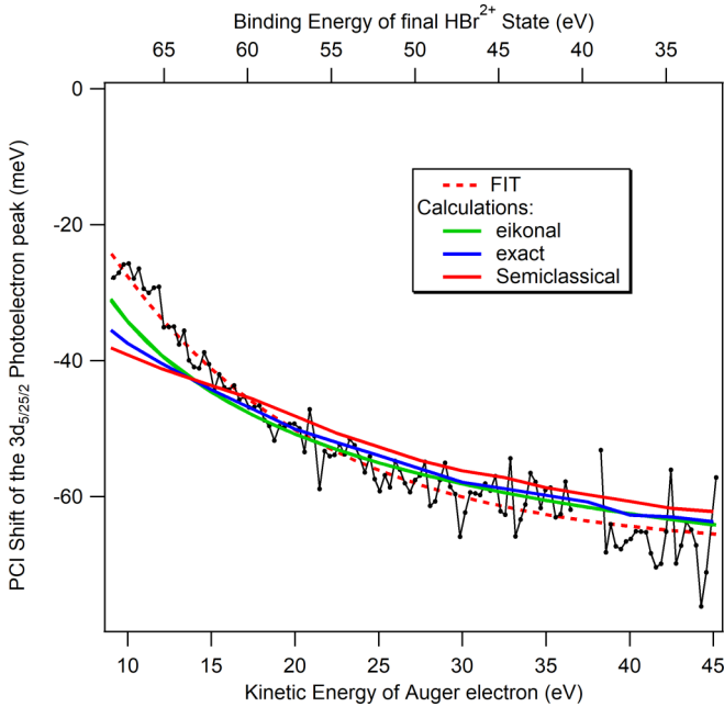
FIG. 6. PCI shift for the 3d_{5/2,5/2}^{-1} photoline as a function of the Auger kinetic energy. The black dots are experimental values obtained from the fit (see text). The red dotted line is a fitted curve to guide the eye. The solid lines give the PCI dependence predicted by three different models, namely, eikonal approximation [31], semiclassical approximation [32], and eikonal approximation with an exact account of Auger-electron-photoelectron interaction [54]. The absolute experimental energy error bar is estimated as \pm 30 meV. Scatter of the data points suggests that the relative error bar is smaller at \pm 3 meV. Photon energy used in the theoretical estimation was set at 81.05 eV. For details, see text.
