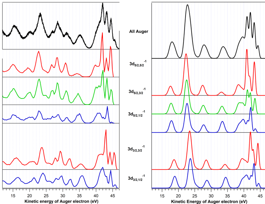
FIG. 4. Total Auger spectrum (top) and its decomposition into the individual Auger spectra of each \text{Br } 3d^{-1} component. The left panel displays the experimental results obtained from the fit analysis of the diagonal lines in Fig. 1(c) and the right panel displays the present theoretical results. For details, see text.
