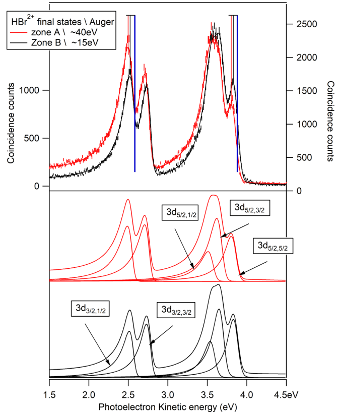
FIG. 2. PCI distortion of the Br 3d^{-1} photoelectron lines. The upper panel shows the 3d^{-1} photoelectron lines measured in coincidence with Auger electrons in given kinetic-energy ranges so that well-defined final states of \text{HBr}^{2+} are populated. The red curves represent data in coincidence with Auger electrons from zone A in Fig. 3, corresponding to an Auger electron of \approx 40 eV and the final state 4p\sigma^{-1}4p\pi^{-1}({}^{1,3}\Pi) . The black curves are related to zone B, i.e., Auger electrons of \approx 15 eV leading to highly excited states of \text{HBr}^{2+} . The experimental error bars represent only the statistical uncertainties. The solid lines represent the result of a fit analysis taking into account the PCI distortion (see text). The vertical bars mark the positions of the maxima of the PCI-distorted 3d_{3/2,1/2}^{-1} and 3d_{5/2,5/2}^{-1} photoelectron lines, and their expected position in the absence of PCI effect (broad blue vertical line). The lower two panels give the individual PCI distorted contributions deduced from these fits.
