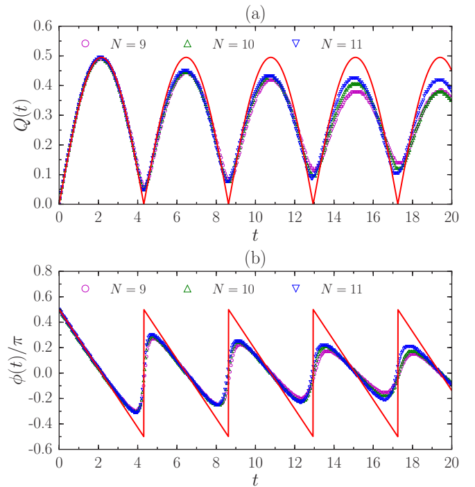
FIG. 12. Exact dynamics of (a) Q and (b) \phi for N = 9-11 fermions at \nu = 1/3 with the V_1 interaction. The adiabatic geometric quench is driven by choosing A_0 = 0 and A_1 = \ln 1.3 . The red solid curve is the Q \geq 0 part of Eqs. (5) and (6), with A \approx 0.248 and E_\gamma \approx 1.457 . These two parameters are obtained by fitting the first oscillation of Q of N = 11 against the solution.
