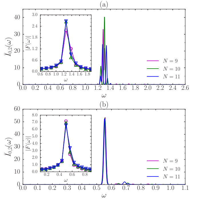
FIG. 5. Normalized spectral function \bar{I}_{0,2}(\omega) = I_{0,2}(\omega)/\int I_{0,2}(\omega)d\omega for isotropic systems of N = 9 – 11 bosons at \nu = 1/2 with (a) contact and (b) Coulomb interactions. The insets show the discrete Fourier transform |F(\omega)| of Q in Figs. 3 and 4. Markers in insets and curves in main figures with the same color refer to the same system size.
