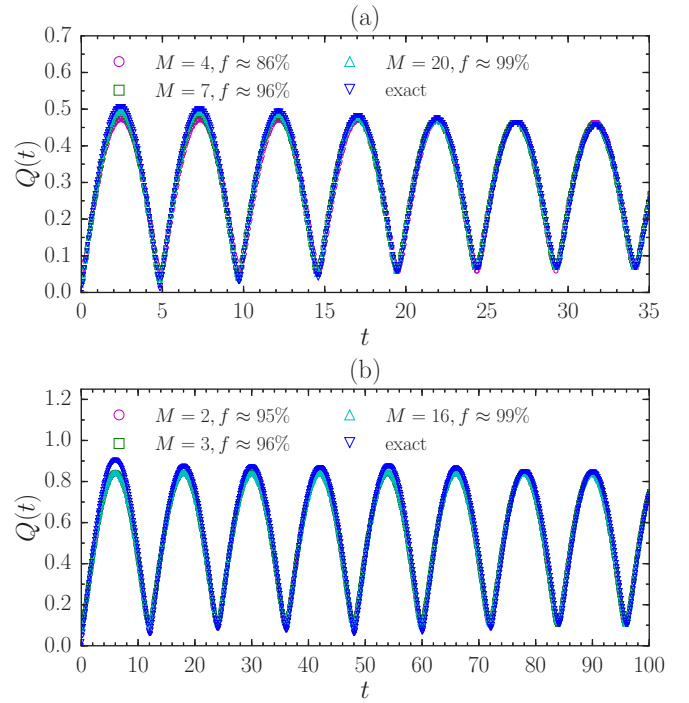
FIG. 10. Dynamics of Q projected to M eigenstates of H' with dominant |\langle n | \hat{V}_{0,2} |0\rangle|^2 . We consider N = 11 bosons at \nu = 1/2 with (a) contact and (b) Coulomb interactions. The quench parameters A_0 and A_1 are the same as those in Figs. 3 and 4, respectively.
