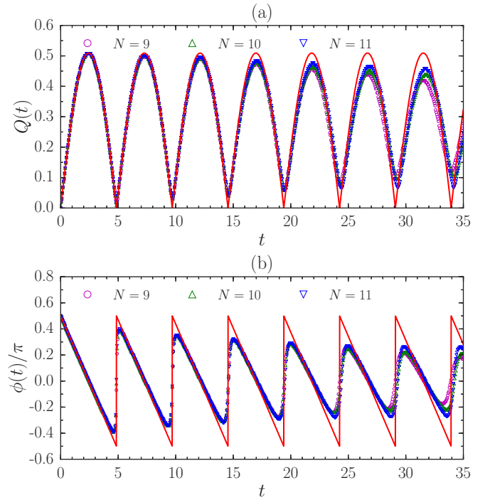
FIG. 3. Exact dynamics of (a) Q and (b) \phi for N = 9 – 11 bosons at \nu = 1/2 with the contact interaction. The quench is driven by choosing A_0 = 0 and A_1 = \ln 1.3 . The red curves are fits to Eqs. (5) and (6), which coincide with the predictions of the bimetric theory, discussed in Sec. V.
