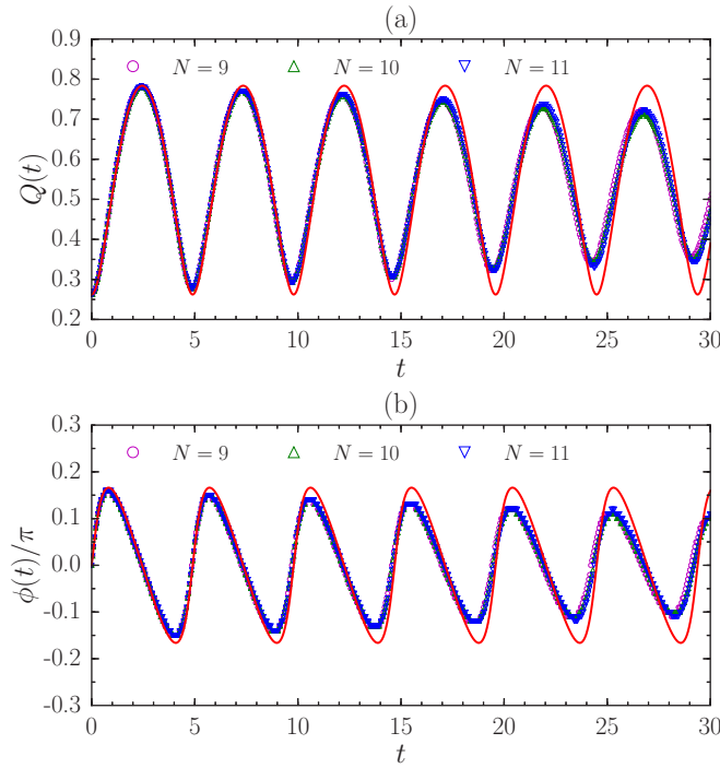
FIG. 9. Exact dynamics of (a) Q and (b) \phi for N = 9-11 bosons at \nu = 1/2 with the contact interaction. The adiabatic geometric quench is driven by choosing A_0 = \ln 1.3 and A_1 = \ln 1.7 . The red solid curve is the solution of linearized equations (20) and (21) under the initial condition Q(0) = A_0 , \phi(0) = 0 , with A \approx 0.523 and E_\gamma \approx 1.283 . These two parameters are obtained by fitting the first oscillation of Q of N = 11 against the solution.
