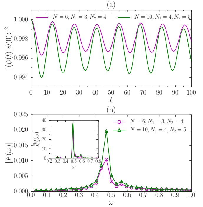
FIG. 14. (a) Dynamics of fidelity, |\langle \psi(t) | \psi(0) \rangle|^2 , and (b) its discrete Fourier transform for \nu = 1/2 bosonic Laughlin FCIs. The adiabatic quench is driven by \alpha' = 15^\circ . The inset of (b) shows the normalized spectral function \bar{I}_{0,2}^{\text{lat}}(\omega) = I_{0,2}^{\text{lat}}(\omega) / \int I_{0,2}^{\text{lat}}(\omega) d\omega for the isotropic case with \alpha = 0 . Markers in insets and curves in main figures with the same color refer to the same system size.
