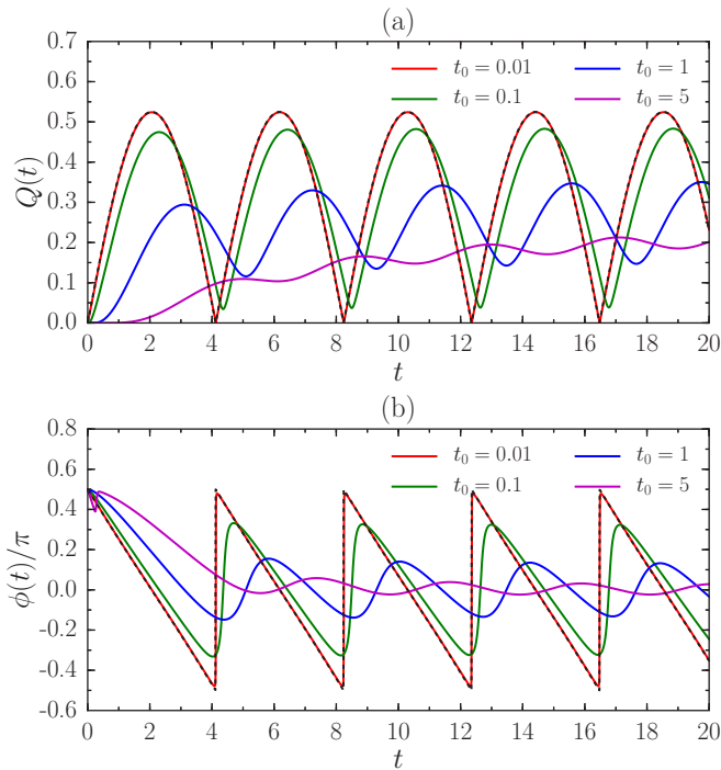
FIG. 11. Solutions of the full equations [Eqs. (15) and (16)] for the noninstantaneous quench with A(t) = A_1 \exp(-t_0/t) , under the initial condition Q(0) = 0 . Here we focus on the Q \geq 0 solution. We choose \Omega = 1.5/4 , \gamma = -1 , A_1 = \ln 1.3 , and consider several different t_0 = 0.01, 0.1, 1, \text{ and } 5 . For comparison, we also give solutions for the instantaneous quench as black dashed lines.
