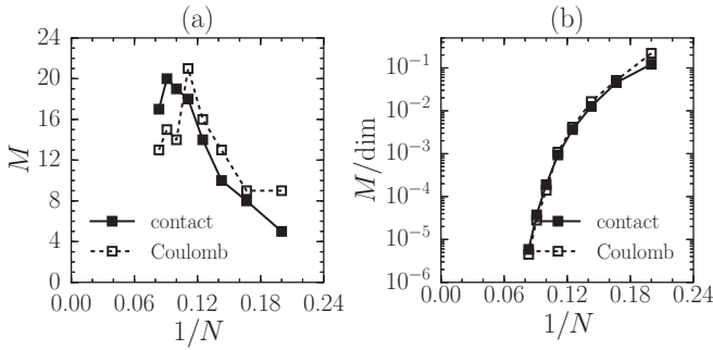
FIG. 6. Finite-size scaling of the number of spin-2 states in the \mathbf{k} = 0 Hilbert space for N = 5\text{--}12 bosons at \nu = 1/2 . M represents the number of states which contain f = 99\% of the total |\langle n | \hat{V}_{0,2} | 0 \rangle|^2 . We consider both contact and Coulomb quench Hamiltonians, with A_1 = \ln 1.3 and A_1 = \ln 2.0 , respectively. The plots show (a) M and (b) M/\text{dim} , where \text{dim} is the \mathbf{k} = 0 Hilbert space dimension.
