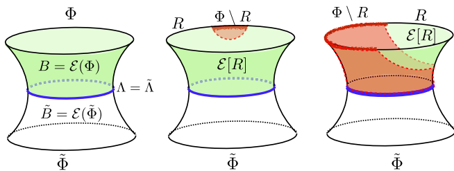
FIG. 2. The left diagram illustrates the thermofield double construction, in which a bulk manifold B with logical boundary \Lambda is extended to two copies of B with their logical boundaries identified. This doubled manifold B\tilde{B} describes two holographic codes whose logical systems are maximally entangled. The other two diagrams illustrate that, for a boundary region R contained in the physical boundary \Phi of B , the corresponding minimal surface lies in B .
