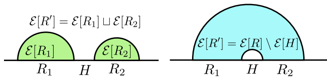
FIG. 4. Two possible geometries for the entanglement wedge \mathcal{E}[R'] of a boundary region R' = R_1 \sqcup R_2 with two connected components separated by the interval H . In the left diagram, the minimal surface is \chi_{R'} = \chi_{R_1} \sqcup \chi_{R_2} , and the entanglement wedge is \mathcal{E}[R'] = \mathcal{E}[R_1] \sqcup \mathcal{E}[R_2] . In the right diagram, the minimal surface is \chi_{R'} = \chi_R \sqcup \chi_H , where R = R_1 H R_2 , and the entanglement wedge is \mathcal{E}[R'] = \mathcal{E}[R] \setminus \mathcal{E}[H] .
