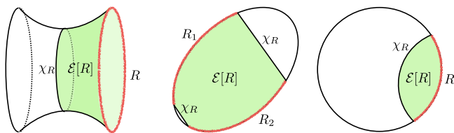
FIG. 1. Geometric notions of minimal surface and entanglement wedge. In each diagram, we highlight a boundary region R with a crayon stroke; the corresponding minimal surface \chi_R is indicated, and the entanglement wedge \mathcal{E}[R] is shaded in green. On the left, B is a hyperboloid whose boundary \partial B has two connected components, where R is one of those components (the one on the right). The minimal surface cuts the hyperboloid at its waist, and the entanglement wedge is everything to the right of \chi_R . In the central diagram, B is the interior of a Euclidean ellipse; the boundary region R = R_1 \sqcup R_2 has two connected components, and \chi_R also has two connected components. As shown, the connected components of \chi_R need not be homologous to R_1 and R_2 , allowing \mathcal{E}[R_1 \sqcup R_2] to be significantly larger than \mathcal{E}[R_1] \sqcup \mathcal{E}[R_2] . On the right, B is the Poincaré disc, portraying an infinite hyperbolic geometry. The minimal surface is a geodesic in the bulk with end points on \partial B .
