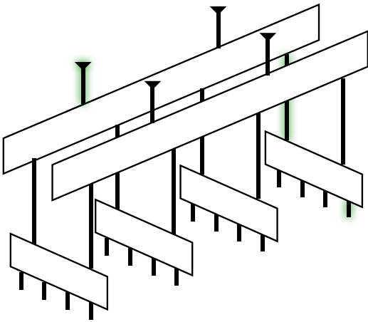
FIG. 6. A recursive coding network to which Eqs. (A3) and (A4) apply, with logical qubits at the top and physical qubits at the bottom. To derive that the distance is bounded below by d^\ell and the price is bounded above by p^\ell , it suffices to observe that there is a unique “causal” path connecting each physical qubit to each logical qubit. Here, a [[4,2,2]] code (with the encoder drawn as a parallelogram) is concatenated to obtain a [[16,4,4]] code, and a causal path connecting a physical qubit to a logical qubit is highlighted.
