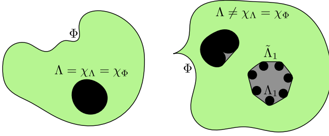
FIG. 3. Necessary condition \chi_\Lambda = \Lambda for the interior boundary of a Riemannian manifold B to be identified as a logical system. In both diagrams, the physical Hilbert space \mathcal{H} resides on the exterior boundary \Phi of B , and \Lambda is the boundary of the punctures in the bulk, which are shaded in black. The green region is the entanglement wedge \mathcal{E}[\Phi] , bounded by \Phi and the minimal surface \chi_\Phi = \chi_\Lambda separating \Phi from \Lambda ; the gray region is B \setminus \mathcal{E}[\Phi] . For purposes of illustration, we assume the bulk metric is Euclidean. On the left, we have \chi_\Lambda = \Lambda , and the interpretation of \Lambda as a logical system is consistent. On the right, we have \chi_\Lambda \neq \Lambda , and two possible reasons for this are illustrated. First, a connected component of \Lambda may fail to be convex. Second, the union \Lambda_1 of several connected components of \Lambda may be encapsulated by a surface \tilde{\Lambda}_1 with smaller area than \Lambda_1 , in which case the logical system resides on \tilde{\Lambda}_1 rather than \Lambda_1 . The emergence of this new logical system is reminiscent of the merging of small black holes to form a larger black hole.
