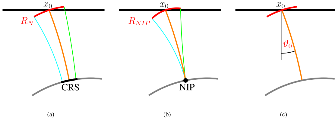
Figure 5. (a) Hypothetic zero-offset experiment: radius of curvature R_N , measured at x_0 , of a wavefront (red) emitted by an exploding curved reflector element (black) denoted CRS (common reflection surface). (b) Hypothetic CMP experiment: radius of curvature R_{NIP} , measured at x_0 , of a wavefront (red) emitted by a point source (black) in the NIP (normal incidence point). A central ray (orange) and two paraxial rays (cyan and green) are also shown. Note that the zero-offset rays are only perpendicular to the reflector (grey) in the isotropic case. In the anisotropic case, normal incidence refers to the slowness, not the ray direction. In the special case of a point diffractor, the radii R_N and R_{NIP} coincide. (c) The ray angle \vartheta_0 lies between the central ray and the vertical direction.
