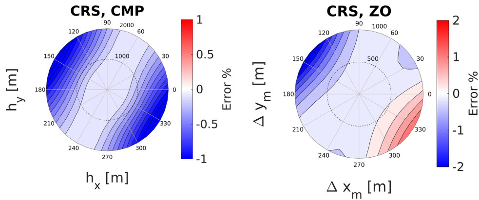
Figure 10. Relative traveltime errors of the anisotropic zero-offset CRS operator for a complex-shaped reflector under a homogeneous overburden with ellipsoidal anisotropy for (a) \Delta x_m = 0 , that is, CMP traveltimes; (b) \Delta h = 0 , that is, zero-offset traveltimes.
