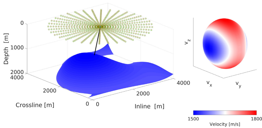
Figure 9. Velocity model for the 3-D example featuring a homogeneous overburden with ellipsoidal symmetry over a complex-shaped reflector. Red and green triangles mark the source and receiver positions. The black line corresponds to the zero-offset ray under consideration.
