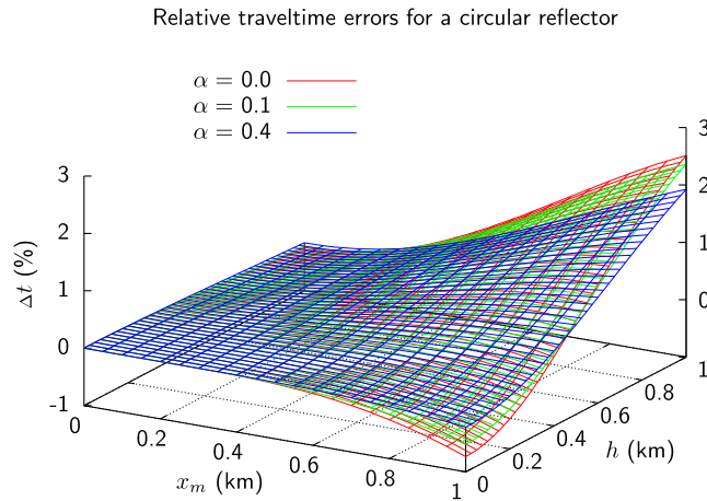
Figure 7. Relative traveltimes errors of the anisotropic zero-offset CRS operator for a circular reflector with a radius of 1 km in a homogeneous medium with elliptical anisotropy. The CMP under consideration is located at x_0 = 0.2 km.
