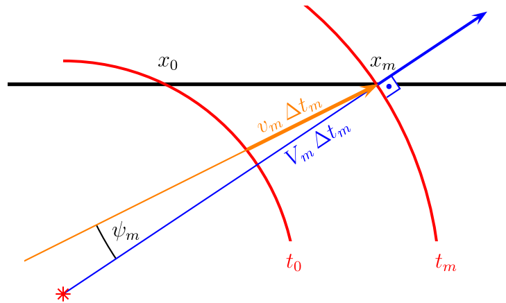
Figure 2. Distances between the wavefronts at x_0 and x_m expressed by the phase and group velocities V_m and v_m , respectively, and the traveltime difference, that is, moveout, \Delta t = t_m - t_0 . The angle \psi_m lies between the slowness and ray direction. It relates the phase and group velocities by V_m = v_m \cos \psi_m .
