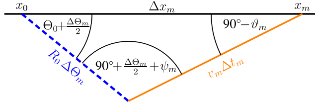
Figure 3. Triangle for the law of sines (see the text). The additional contribution of \Delta\Theta_m/2 results from the projection of the wavefront element onto the straight line R_0 \Delta\Theta_m .
