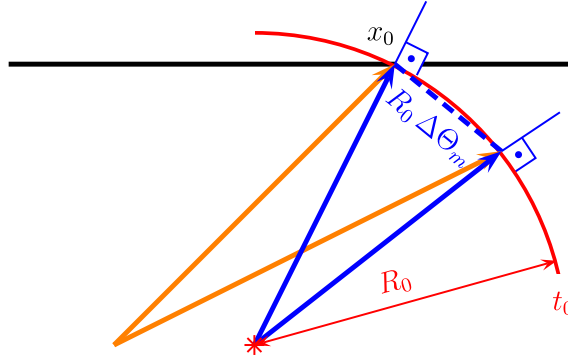
Figure 4. The wavefront segment at x_0 that corresponds to the arc between \Theta_m and \Theta_0 is approximated by the dashed line. Its length is given by R_0 \Delta\Theta_m , where \Delta\Theta_m = \Theta_m - \Theta_0 .
