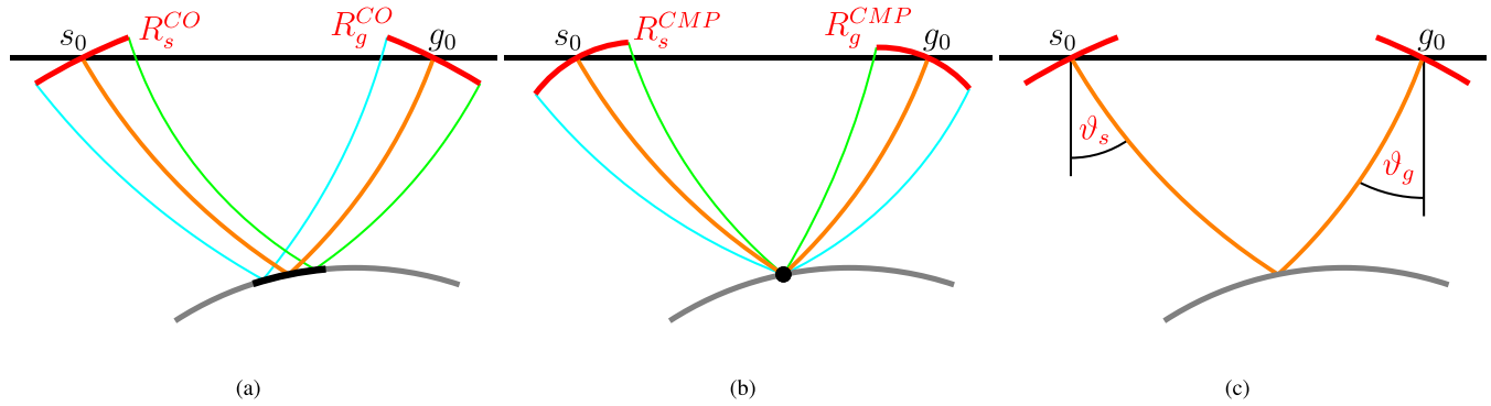
Figure 6. (a) Hypothetic finite-offset experiment: Radii of curvature R_s^{CO} and R_g^{CO} , measured at s_0 and g_0 , respectively, of wavefronts (red) reflected by a curved reflector element (black). (b) Hypothetic CMP experiment: radii of curvature R_s^{CMP} and R_g^{CMP} , measured at s_0 and g_0 , respectively, of wavefronts (red) associated with a common reflection point (black). A central ray (orange) and two paraxial rays (cyan and green) are also shown. (c) The ray angles \vartheta_s and \vartheta_g , respectively, lie between the central ray and the vertical direction.
