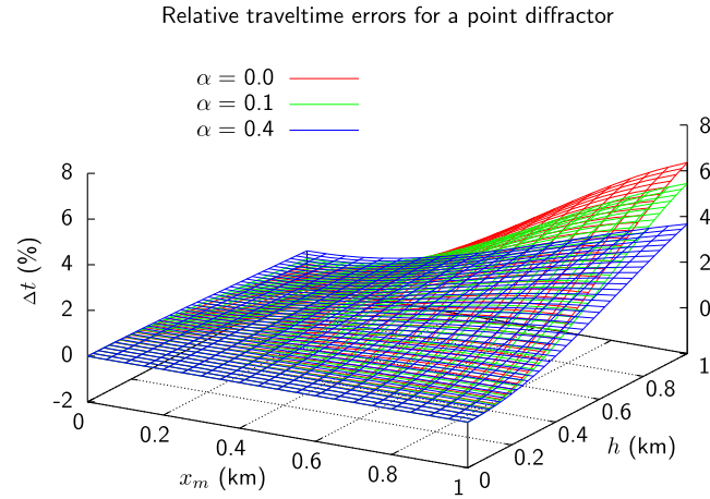
Figure 8. Relative traveltime errors of the anisotropic zero-offset CRS operator for a point diffractor in a homogeneous medium with elliptical anisotropy. The CMP under consideration is located at x_0 = 0.2 km.
