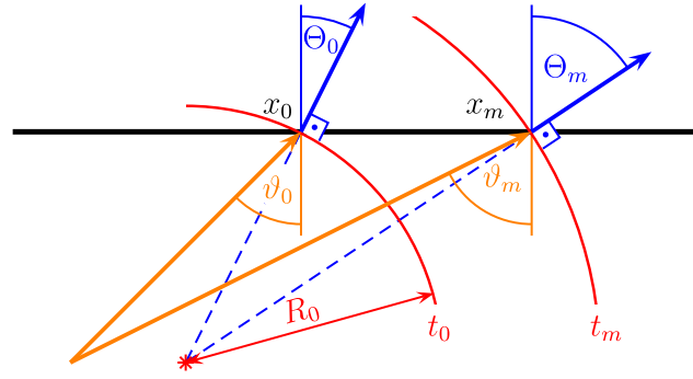
Figure 1. Rays (orange), slowness directions (blue) and their corresponding angles at x_0 and x_m . Wavefronts (red) at the times t_0 (with radius R_0 ) and t_m are locally approximated by circles. Unlike the rays, the slownesses are perpendicular to the wavefronts. The red star marks the hypothetic centre of the wavefront.
