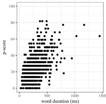
Figure 5: P-scores as a function of word duration
