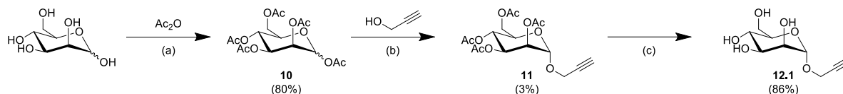
Scheme 3. Synthesis of Man analog 12.1.
