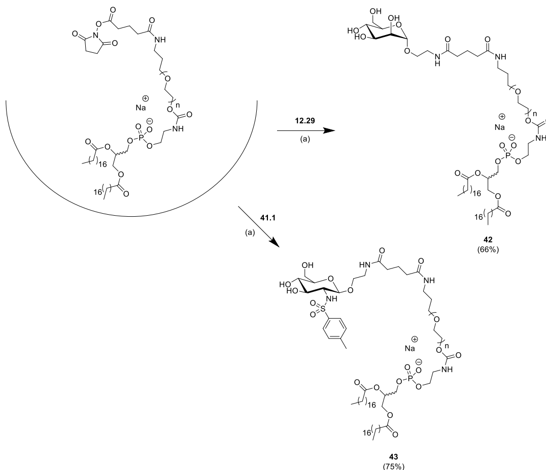
Scheme 8. Synthesis of glycolipids 42 and 43 . 37
