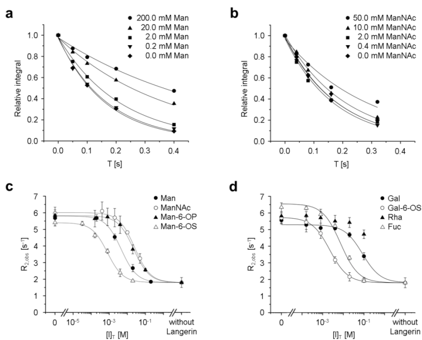
Figure 9. K_I determination for selected monosaccharides.
