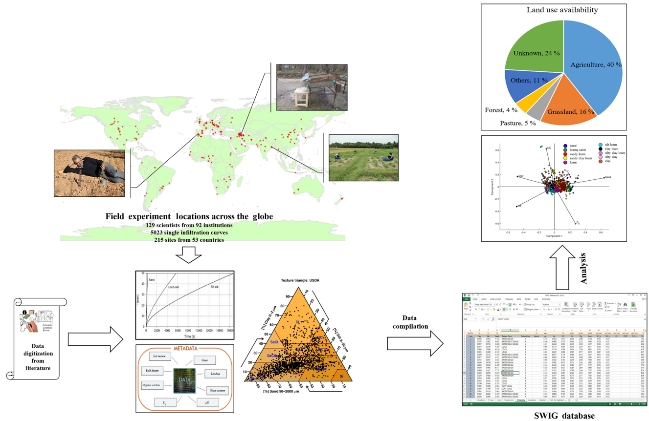
Figure 1. SWIG flowchart.
