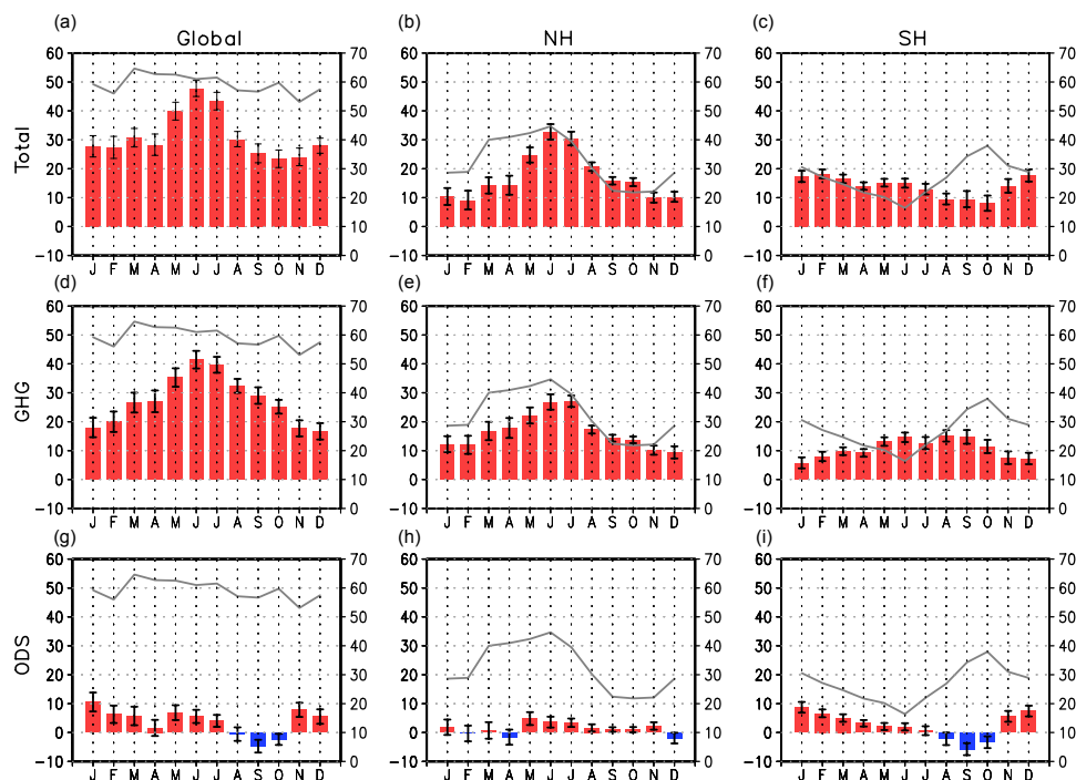
Figure 5. Annual cycle of ozone mass flux changes between 2000 and 2100 [ \text{Tg month}^{-1} ] in the time-slice simulations integrated globally (a, d, g), over the Northern Hemisphere (b, e, h), and over the Southern Hemisphere (c, f, i) for the changes due to all forcings (a–c), for the effect of increasing GHG concentrations (d–f) and for the impact of declining ODS levels (g–i). The black error bars denote \pm 2\sigma . The absolute ozone mass flux of the reference simulation REF2000 is shown as grey line with the corresponding y axis on the right.
