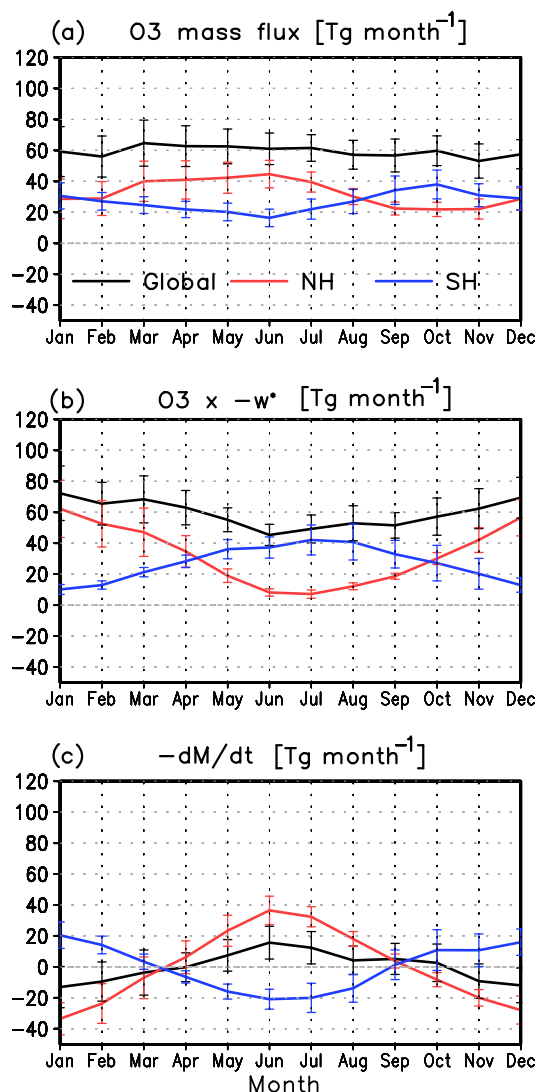
Figure 2. (a) Annual ozone mass flux and its 95 % confidence interval (i.e., \pm 2\sigma , where \sigma is standard deviation) [Tg month -1 ] from the stratosphere into the troposphere ( F_{\text{out}} ) in the REF2000 simulation integrated globally (black), over the Northern Hemisphere (red) and the Southern Hemisphere (blue). (b) Same as (a) but for F_{\text{in}} (the product between the ozone concentration and the negative zonal mean residual vertical velocity \bar{w}^* at 91 hPa). (c) Same as (a) but for the negative monthly change in ozone mass of the LMS ( -dM/dt ), also referred to as seasonal breathing.
