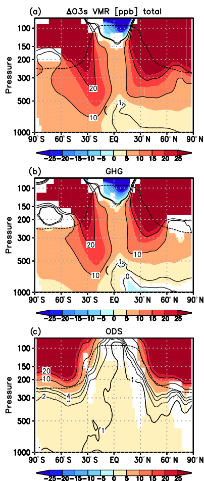
Figure 8. Changes in the volume mixing ratios [ppbv] of the diagnostic tracer O_3s for (a) the changes between 2000 and 2100 due to all forcings, (b) the changes between 2000 and 2100 due to increasing GHG concentrations and (c) the changes between 2000 and 2100 due to declining ODS levels for June (when the ozone mass flux is maximum in the NH and minimum in the SH; see Fig. 2a). Significant changes at the 95 % confidence level are colored. The black dotted line represents the mean tropopause position in the REF2000 simulation. For the small ODS-induced changes (c) additional contour lines (2, 3, and 4 ppbv) are shown.
