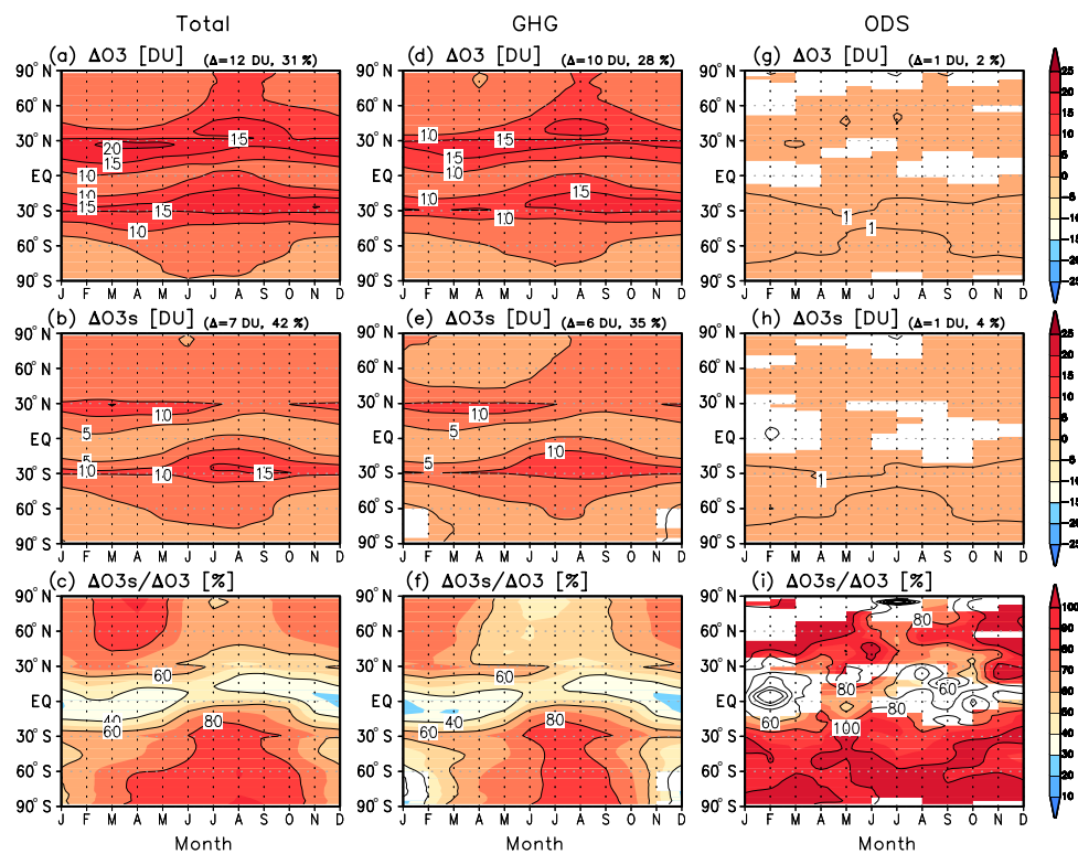
Figure 9. Same as Fig. 6, but for the change in the tropospheric columns of O_3 [DU] (a, d, g), the tropospheric columns of O_3s [DU] (b, e, h), and the contribution of the O_3s changes to the O_3 changes between 2000 and 2100 [%] (c, f, i). The small numbers on top of the figures are the respective annual mean and global mean changes in Dobson units and percent. Shading in the bottom row indicates the regions where both O_3s and O_3 changes are significant at the 95 % confidence level.
