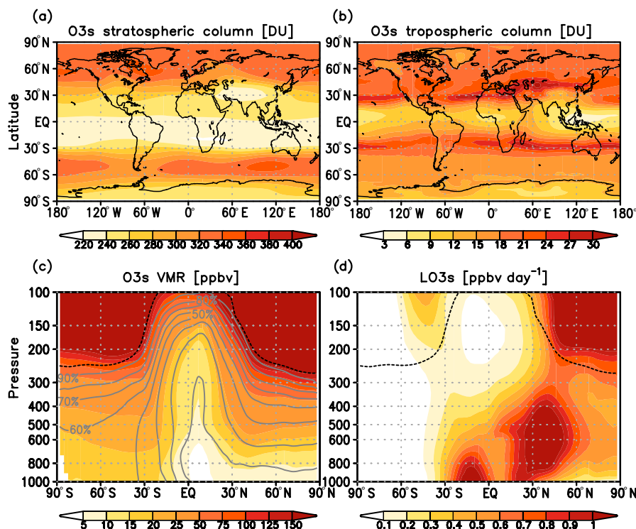
Figure 3. (a) Geographical distribution of stratospheric partial columns of the diagnostic O 3 s tracer in Dobson units (DU) in June for the REF2000 simulation. (b) Same as (a) but for tropospheric columns. (c) Latitude–height section of the O 3 s volume mixing ratios [ppbv] and (d) latitude–height section of the chemical loss rate of O 3 s [ppbv day -1 ]. The black dashed line indicates the position of the mean tropopause. Gray contour lines in (c) show the relative contribution of O 3 s to the ozone field in percent.
