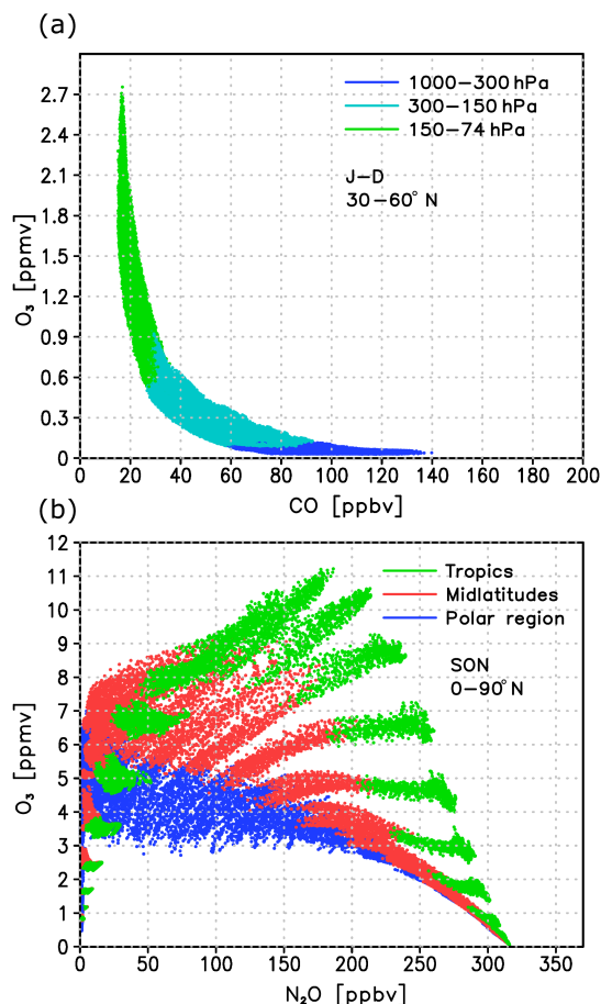
Figure 1. (a) O_3 –CO scatter plot for January to December in the latitude band 30 – 60^\circ N for the REF2000 simulation from the troposphere to the lower stratosphere. Color coding indicates different height regions. (b) O_3 – N_2O scatter plot for September to November in the Northern Hemisphere for the REF2000 simulation at the altitude region between 270 and 0.1 hPa. Color coding indicates different latitude bands.
