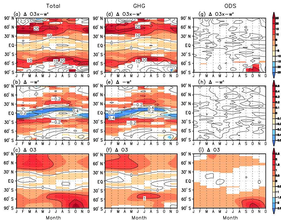
Figure 6. Annual cycle of the zonal mean change at 91 hPa in the time-slice simulations due to all forcings between 2000 and 2100 ( a–c ), due to GHG increase ( d–f ), and due to ODS decrease ( g–i ). ( a, d, g ) Changes in the product of ozone concentration and -\bar{w}^* [ 10^6 \text{ g cm}^{-2} \text{ month}^{-1} ], which equals F_{\text{in}} when integrated over all latitudes. ( b, e, h ) Changes in -\bar{w}^* [ \text{mm s}^{-1} ]. ( c, f, i ) Changes in the ozone concentration [ \text{molecules cm}^{-2} ]. Significant changes at the 95 % confidence level are colored.
