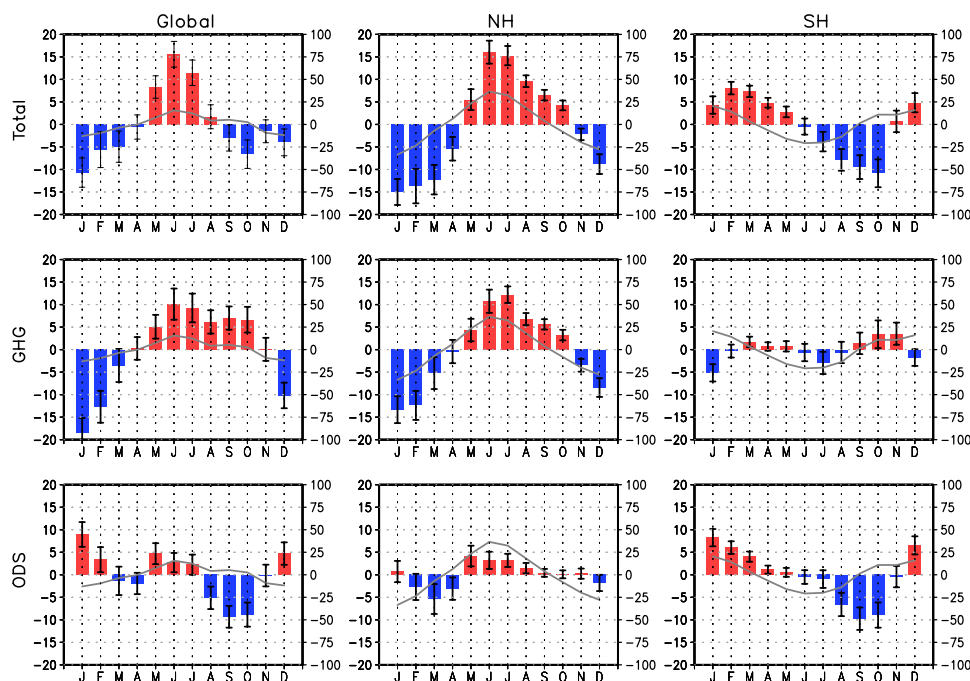
Figure 7. Same as Fig. 5 but for the change in seasonal breathing ( -dM/dt ) [ \text{Tg month}^{-1} ]. The absolute value for -dM/dt of the reference simulation REF2000 is shown as a grey line with the corresponding y axis on the right.
