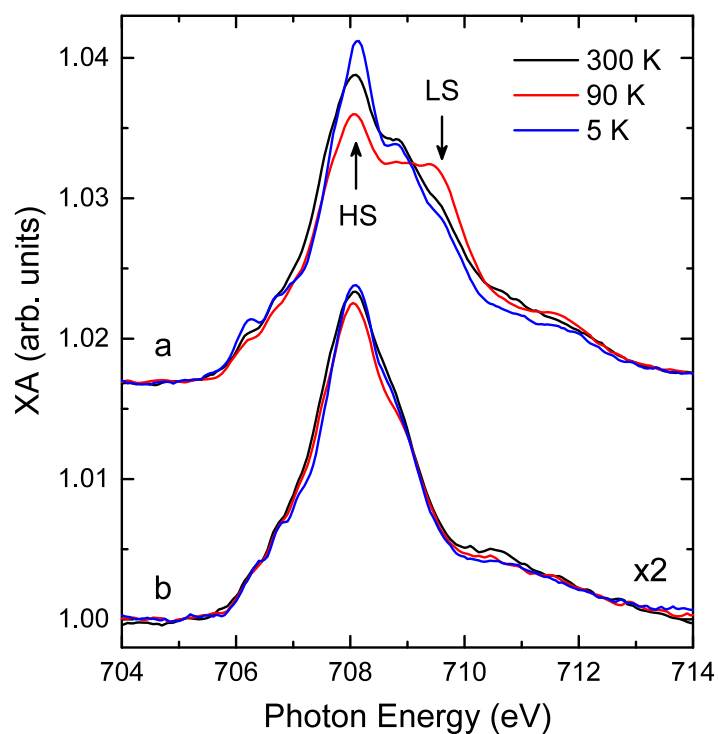
Figure 9. X-ray absorption spectra at the Fe L_3 edge recorded at an angle of incidence of 54.7^\circ at 300, 90, and 5 K of (a) 1.6 ML and (b) 0.8 ML of [\text{Fe}(\text{bpz})_2(\text{phen})] on Au(111). Arrows indicate the energies representative of molecules in the high-spin and low-spin states. While at 0.8 ML coverage the spectra do not change with temperature, at the coverage of 1.6 ML some changes characteristic for a thermal transition from a high-spin state at 300 K towards an increasing content of low-spin state at lower temperatures is observed. After [71], copyright 2013 Wiley-VCH Verlag GmbH & Co.
