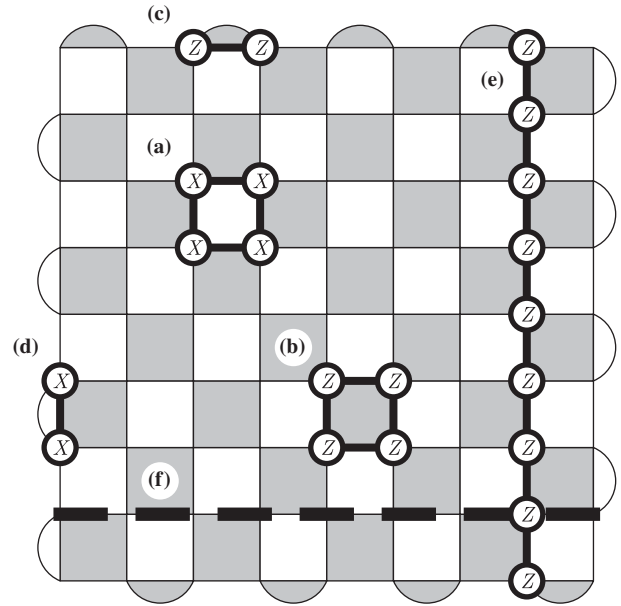
FIG. 1. The planar variant of the surface code with two rough boundaries and two smooth boundaries. Qubits lie on the vertices of the square lattice. Diagrams (a) and (b) show the two different types of weight-four stabilizer operators. Diagrams (c) and (d) show two stabilizers that lie at the boundary of the lattice. (e) The logical operator \bar{Z} is the tensor product of Pauli-Z operators extending from the top to the bottom of the lattice. (f) The logical operator \bar{X} is the tensor product of Pauli-X operators along the horizontal dashed line that extends from the left to the right of the lattice.
